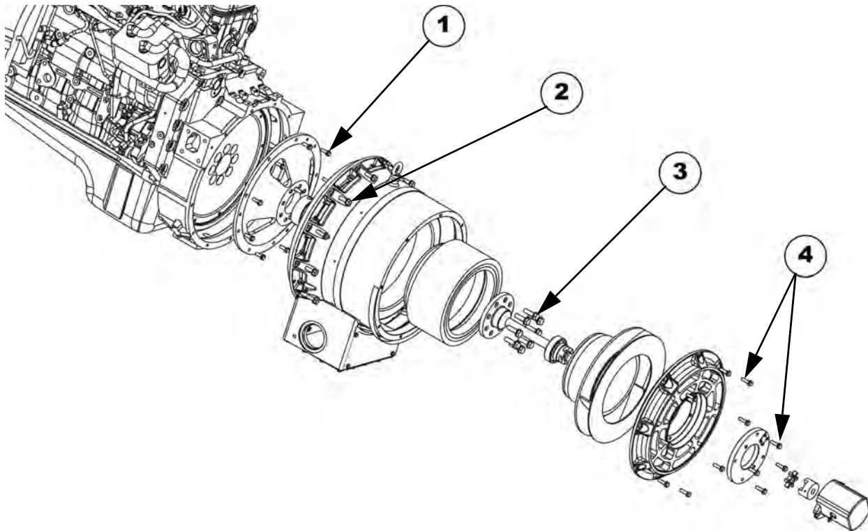
Figure 1-1 Hybrid Generator Critical Torque Spec Locations
