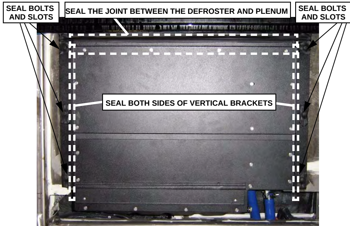
Figure 1-1 Orion VII NG Front Defroster
