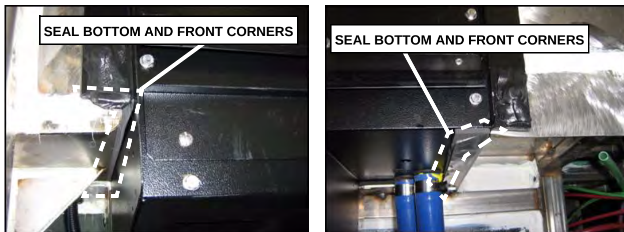
Figure 1-2 Sealing of Bottom and Front Corners
