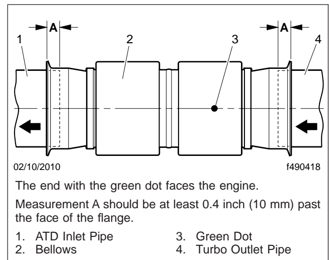
Fig. 6, EPA10 Exhaust Bellows
