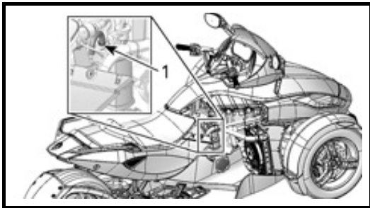
1. Fuel canister vent hose
