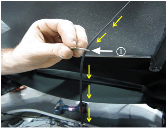
29.2. Route the cord downward through the large eye loop (1) with the eye loop angled downward as shown above.
