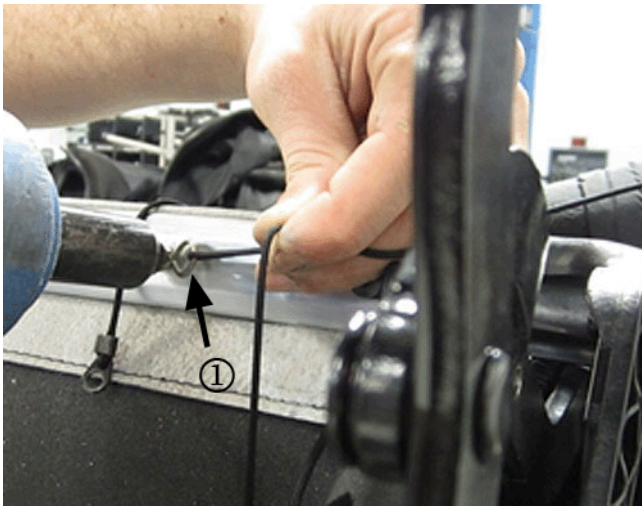
29.3. Install the rivet on the #2 bow through the small eye loop hole with the large eye loop hole (1) aimed outboard as shown above.
