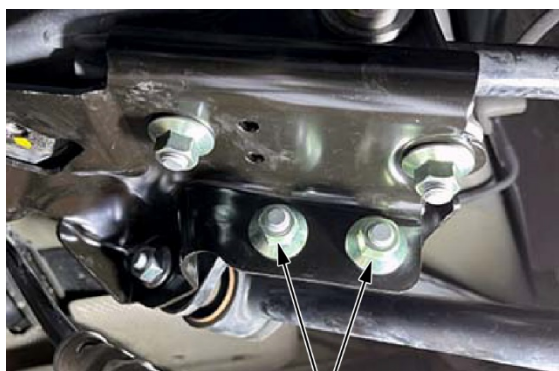
10x30 CARRIAGE BOLTS WITH 10mm FLANGE NUTS
