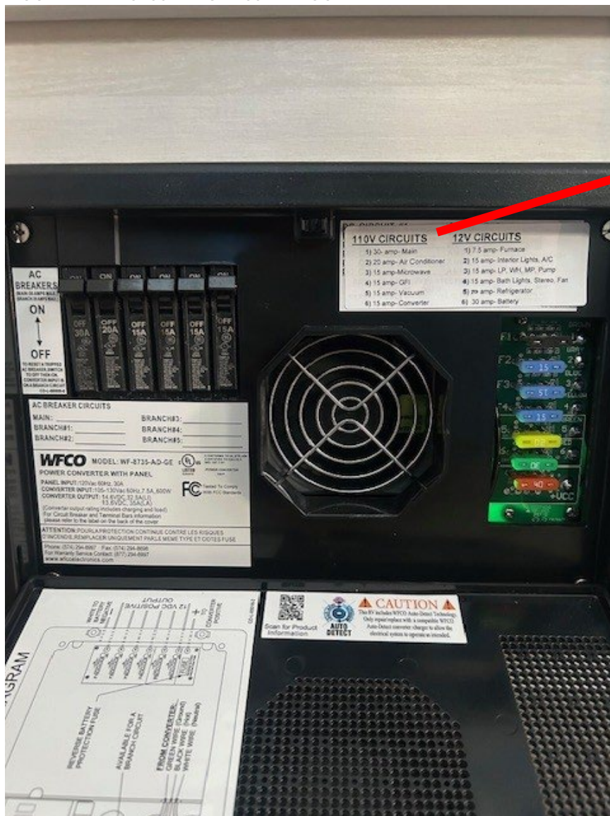
FIGURE 1 - WF-8735-AD-GE - 35 AMP CONVERTER
