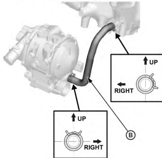
COOLING AIR OUTLET HOSE
