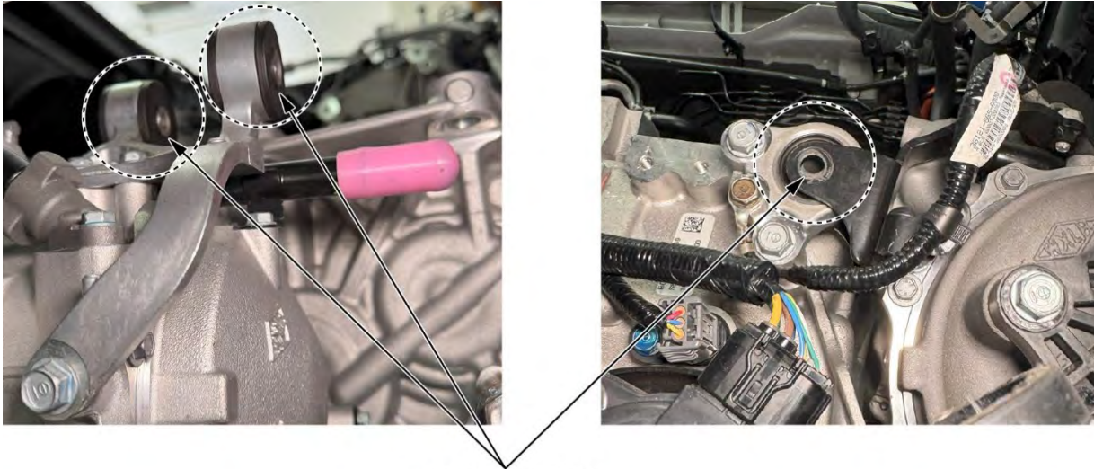
MOUNTING BOLTS
