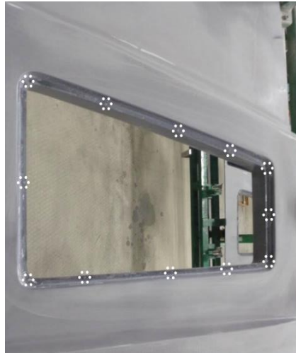
Figure 5: Entrance Door Lower Window Flange
