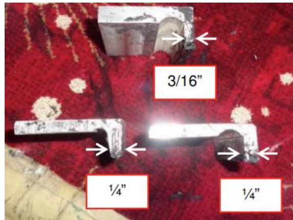
Figure 6: Guiding Spacers to Locate the Window
