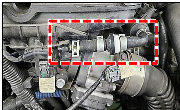
Check Valve
