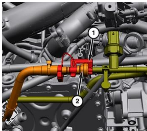
1 - Fuel Line Safety Lock 2 - Fuel Supply Line Quick-Connect Fitting
