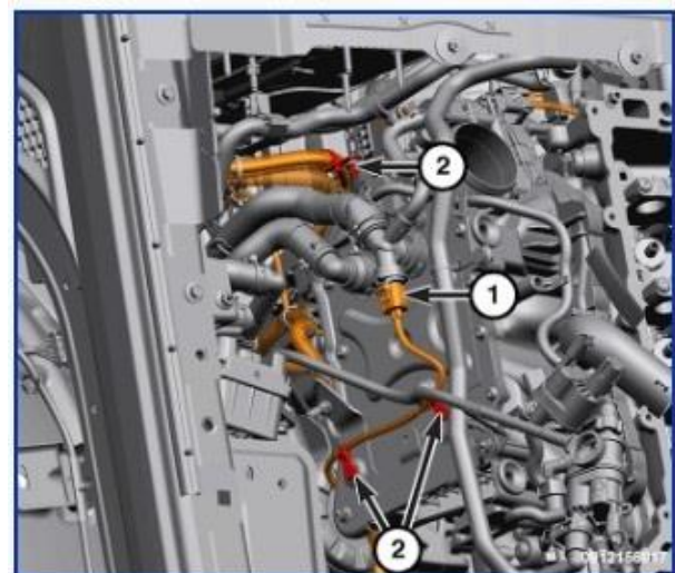
Figure 9 – Coolant Hoses
