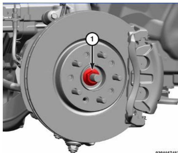
Figure 62 – Halfshaft Nut
