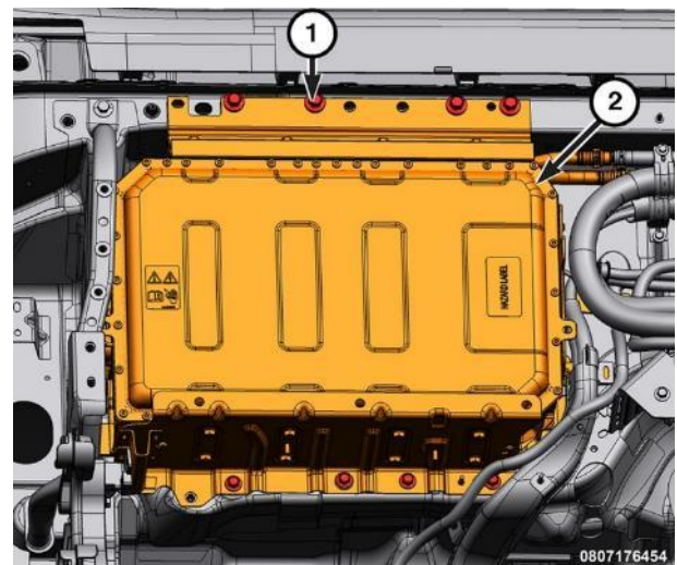
Figure 55 – HV Battery - Secondary
