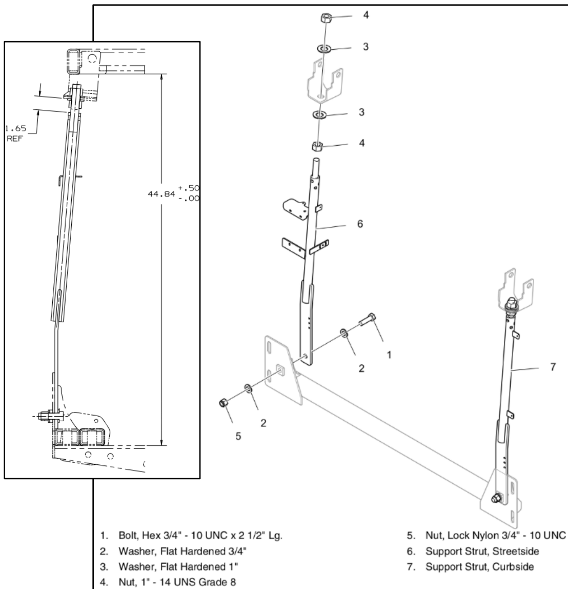
Figure 82: Support Strut Installation
