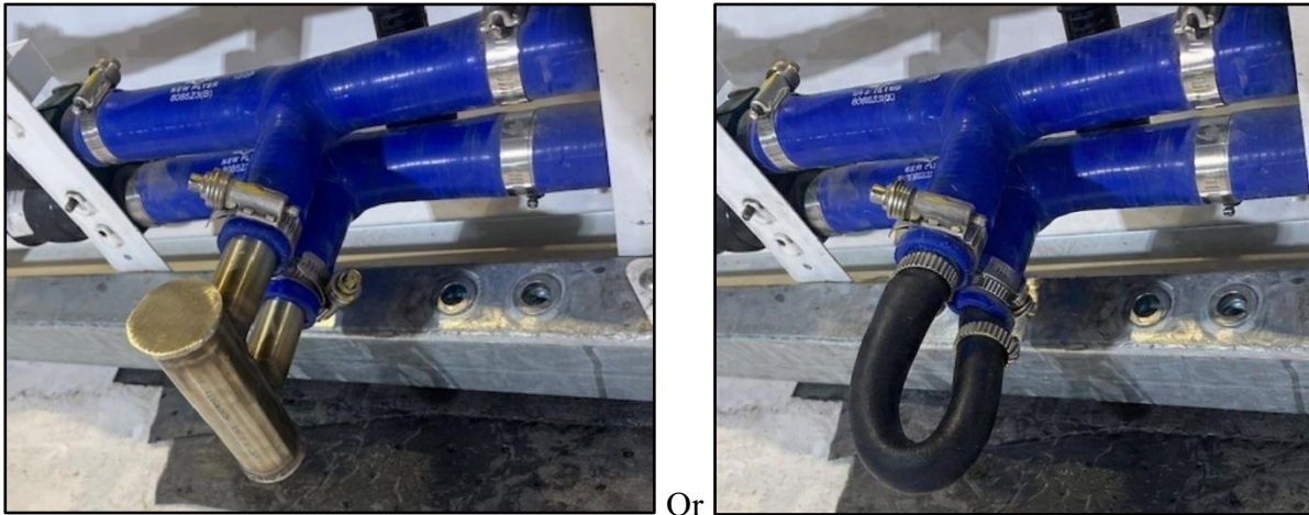
Figure 36: Install U-Shaped Plugs and Clamp on Coolant Hose
