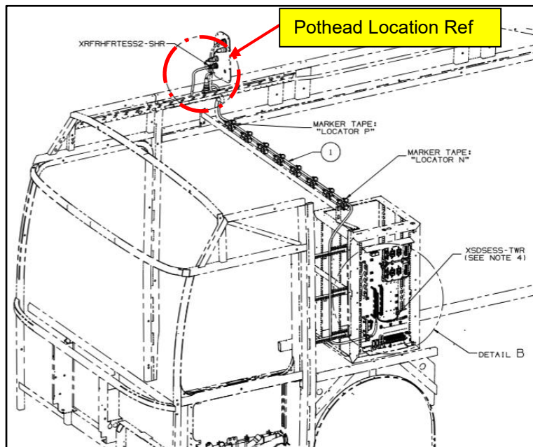
Figure 47: Jumper Harness PN 1147724 Routing Ref
