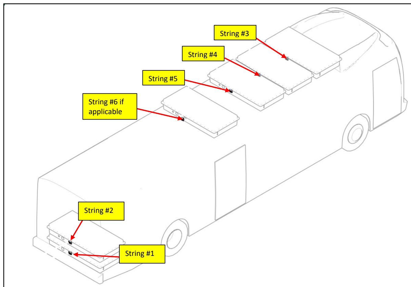
Figure 91: String Location # Reference
