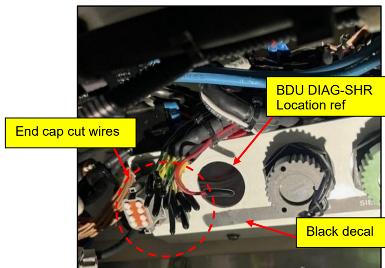
Figure 57: Curbside Rear Bulkhead Harness Rework
