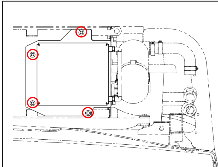
Figure 42: BTMS Surge Tank Mounting Pattern
