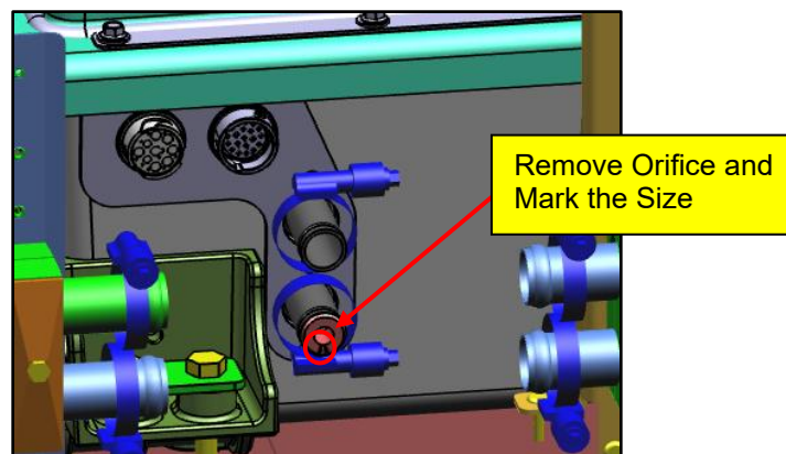
Figure 31: Reducer Orifice on ESS Pack Supply Coolant Port
