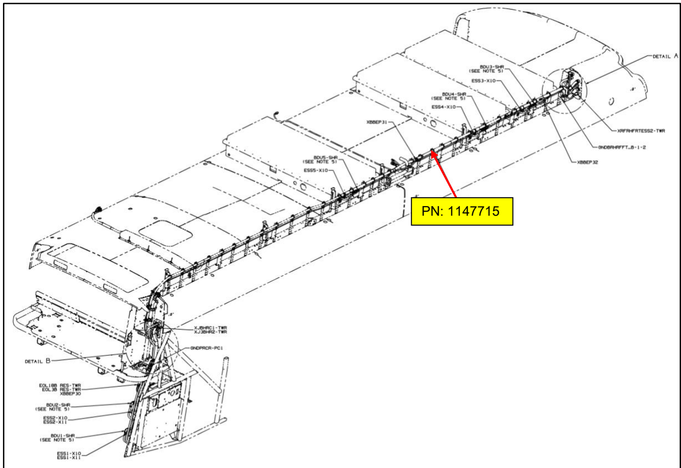
Figure 58: Roof Jumper Harness Routing Reference
