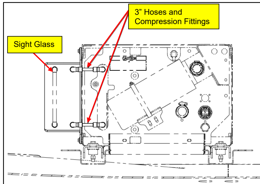
Figure 43: Sight Glass Relocation and Plumbing of BTMS Rework Reference
