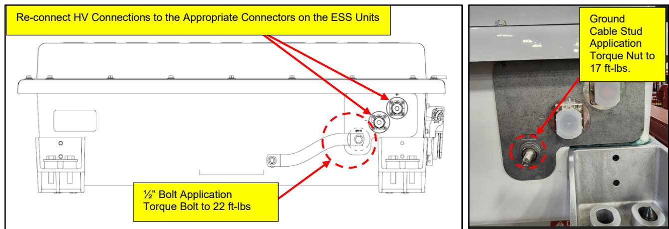
Figure 81: Rear Upper and Lower ESS Assembly Ground Stud and HV Cable Re-installation Location Reference
