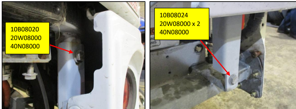
Figure 88a & 88b: Upper and Lower Corner Pillar Mounting Bracket Location Reference
