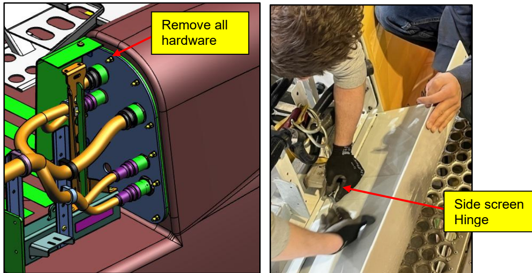
Figure 44a & 44b: Curbside Pothead Plate Removal
