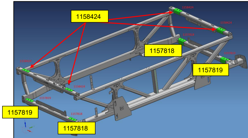
Figure 73: Reinforcement Brackets Added on Existing Rear Rack
