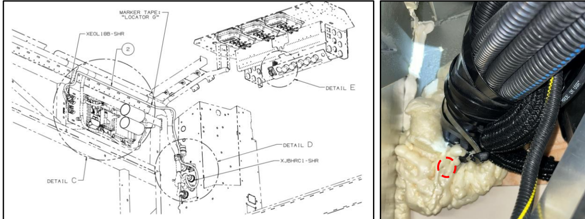
Figure 54a & 54b: Interior Rear Harness Rework
