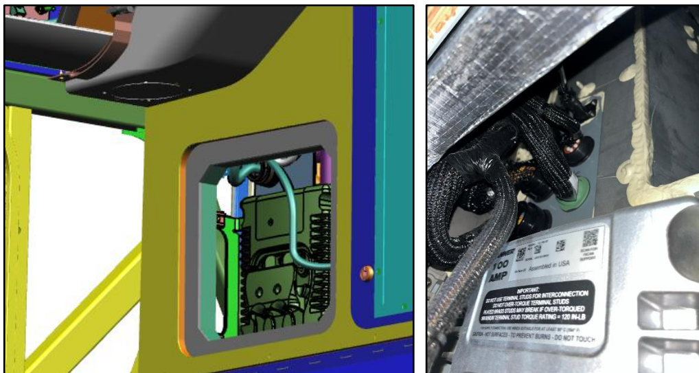
Figure 55a & 55b: Rear CS Access Panel Removed
