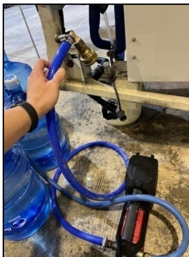
Figure 39: Pressure Fill Hose to the Coupler
