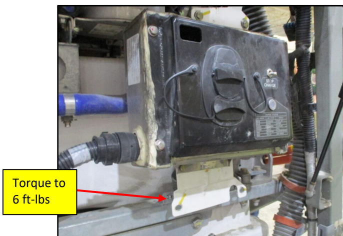
Figure 84: Charger Box Reinstallation
