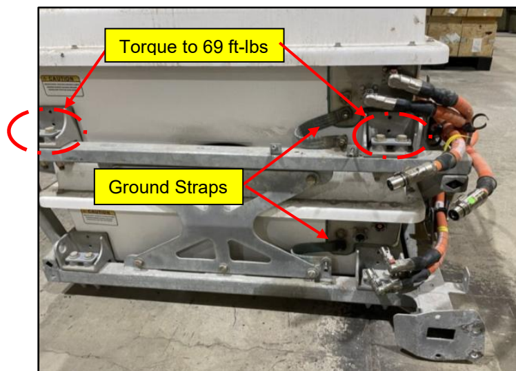
Figure 79: Upper ESS ABS Pack Installation
