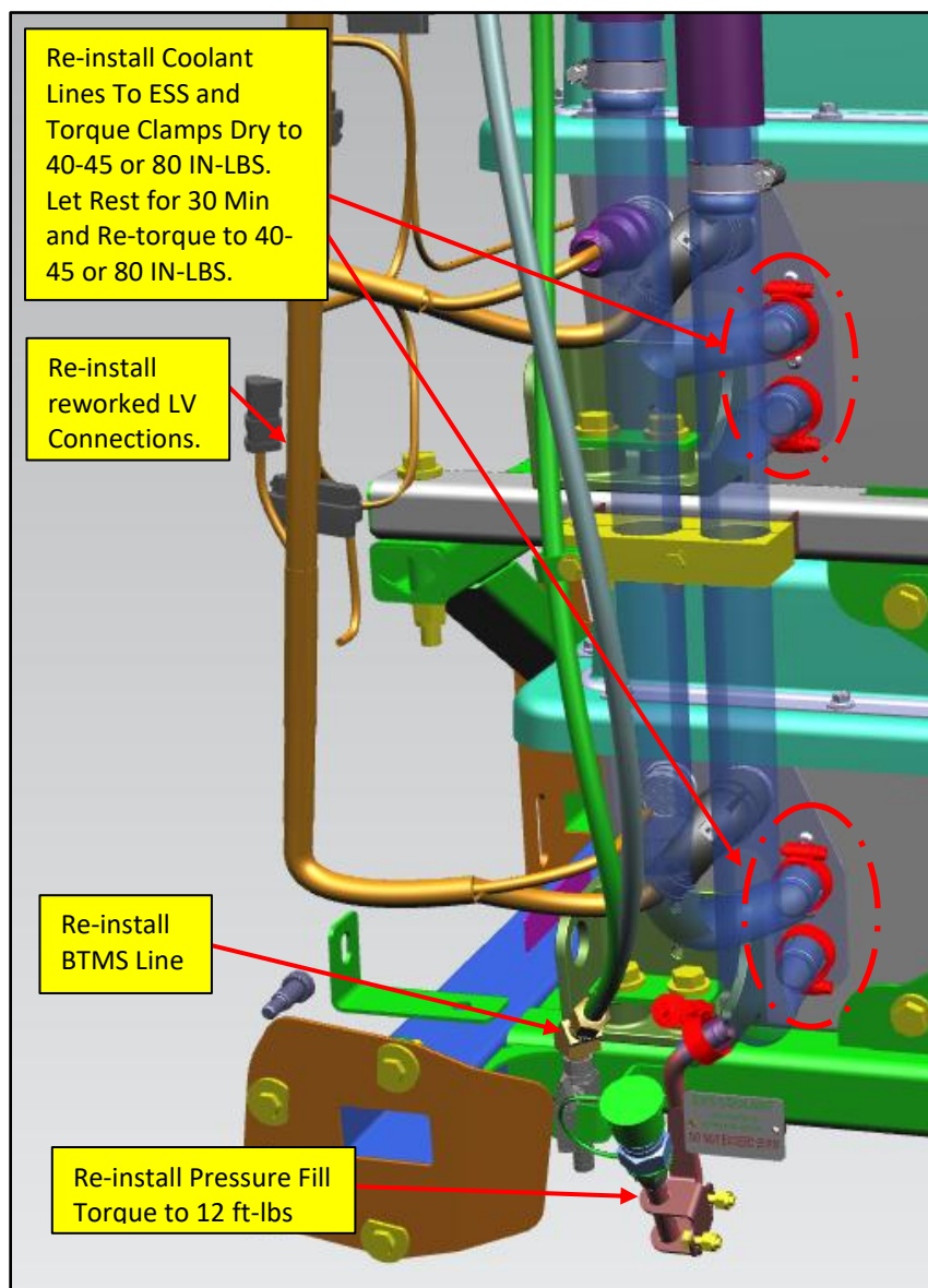
Figure 83: Low Voltage and Coolant Line Connections Location Reference
