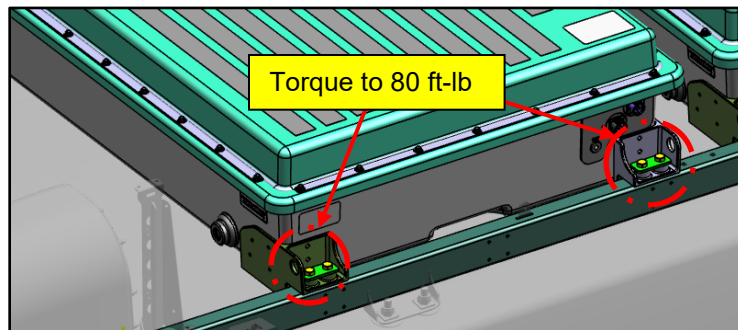
Figure 67: Upper ESS Assembly Installation Location Reference
