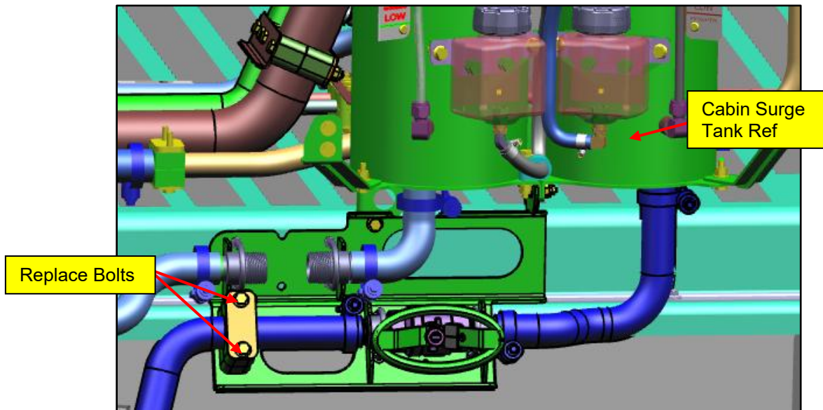
Figure 74: Coolant Hose Clamp under Cabin Surge Tank
