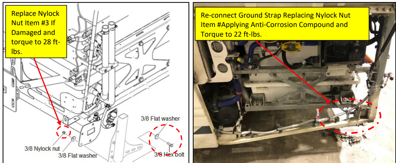
Figure 81: ESS Ground Strap to Bus Frame and Corner Pillar Brackets to Pillar Location Reference
