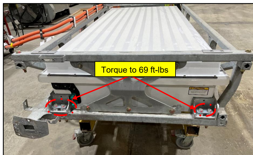
Figure 77: ESS Mounted on Lower Rack Reference
