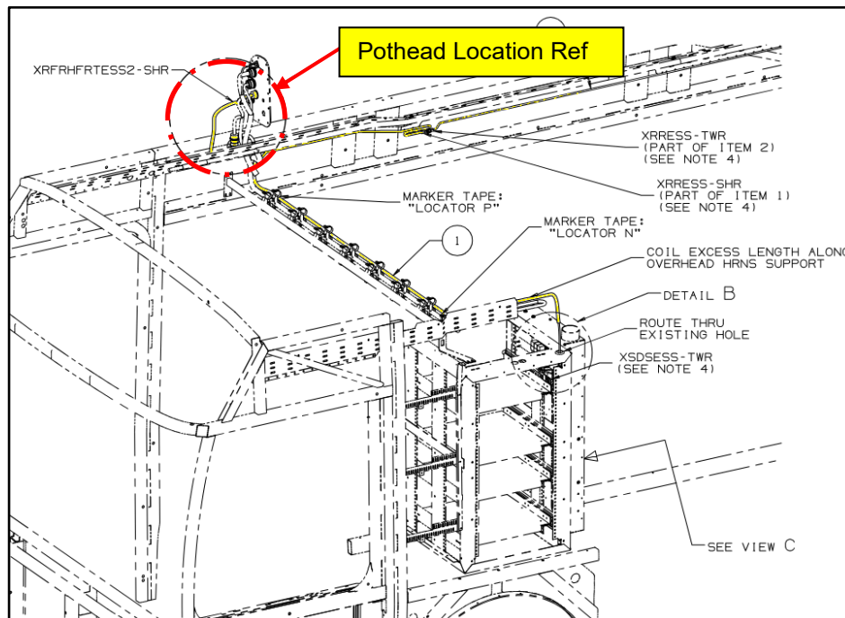
Figure 49: Jumper Harness PN 1166935 Routing Ref
