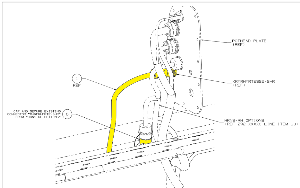
Figure 47: Pothead Interior Side
