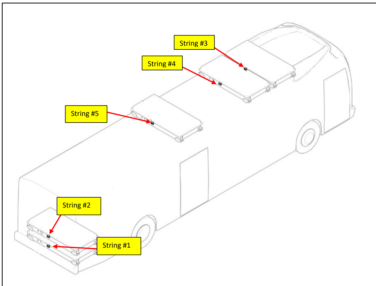
Figure 94: String Location # Reference
