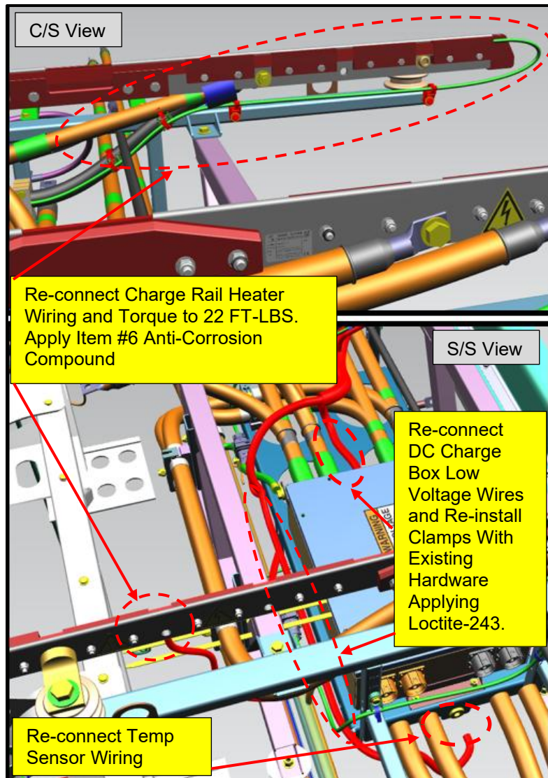
Figure 73c: Charge Rail Installation Location Reference
