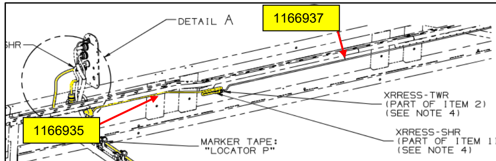
Figure 53: XRRESS Connections from Two Jumper Harness
