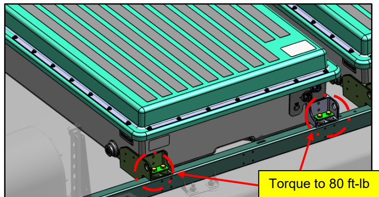
Figure 67: Upper ESS Assembly Installation Location Reference
