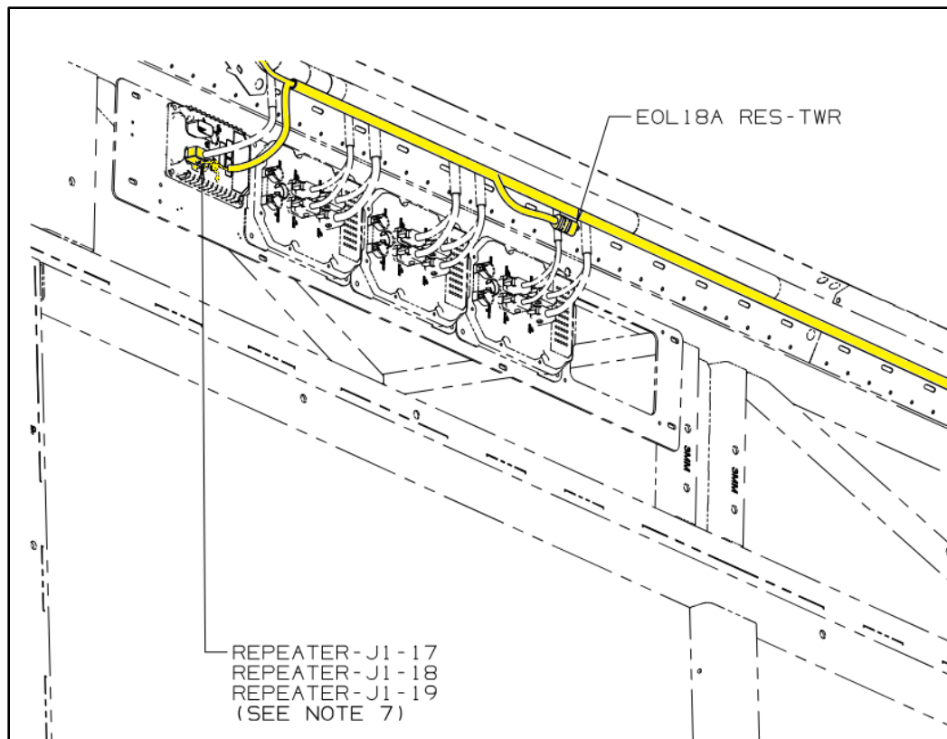
Figure 54: Repeater J1 Connection Location Ref
