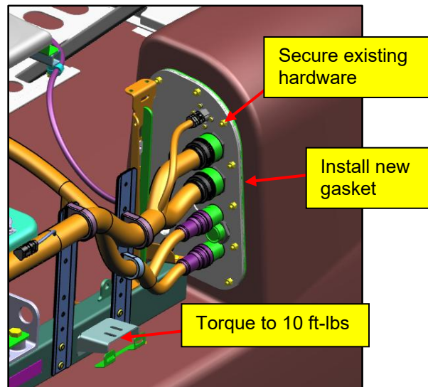
Figure 48: Curbside Pothead Plate Reinstallation
