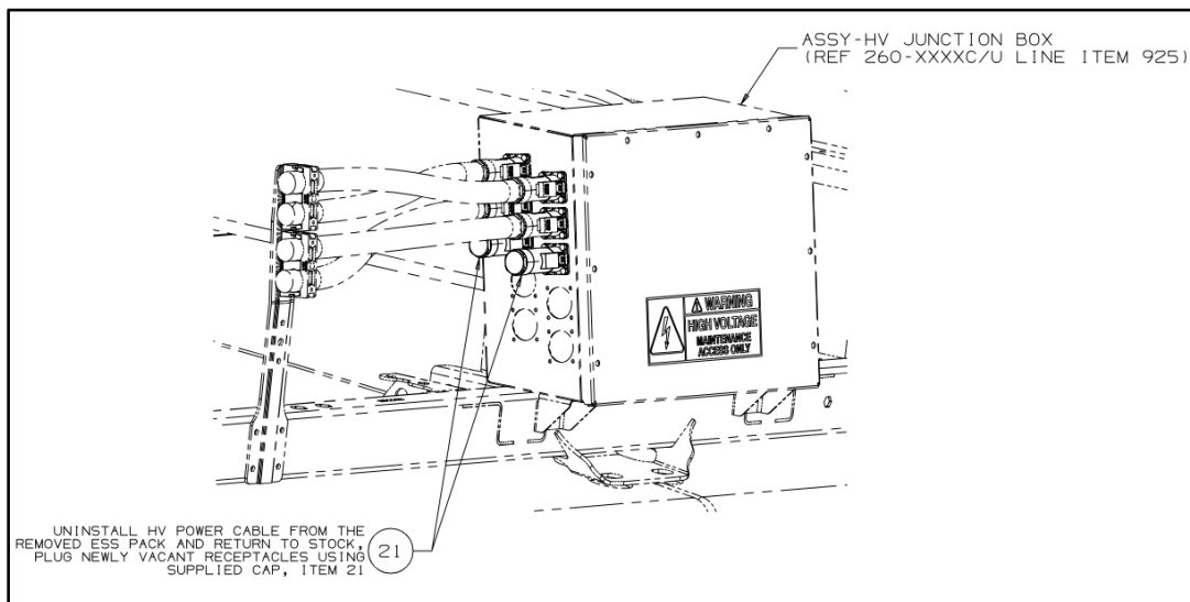
Figure 64: Roof Top HV Junction Box
