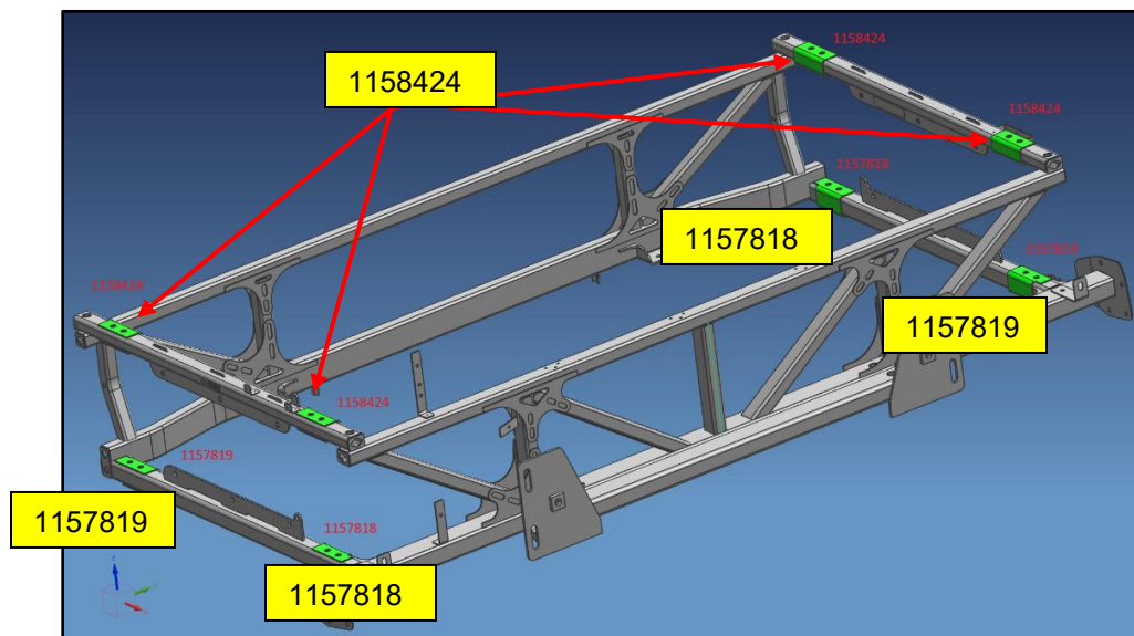
Figure 75: Reinforcement Brackets Added on Existing Rear Rack
