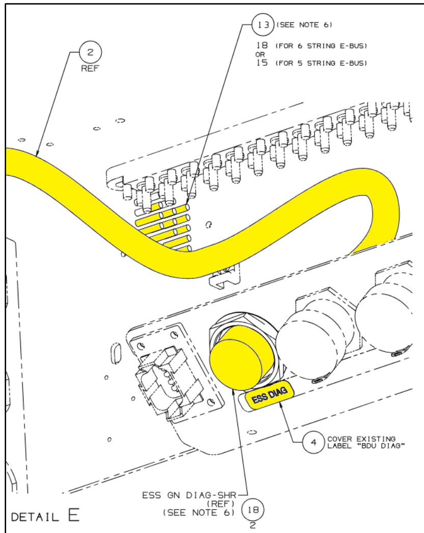
Figure 57: ESS GN DIAG Routing
