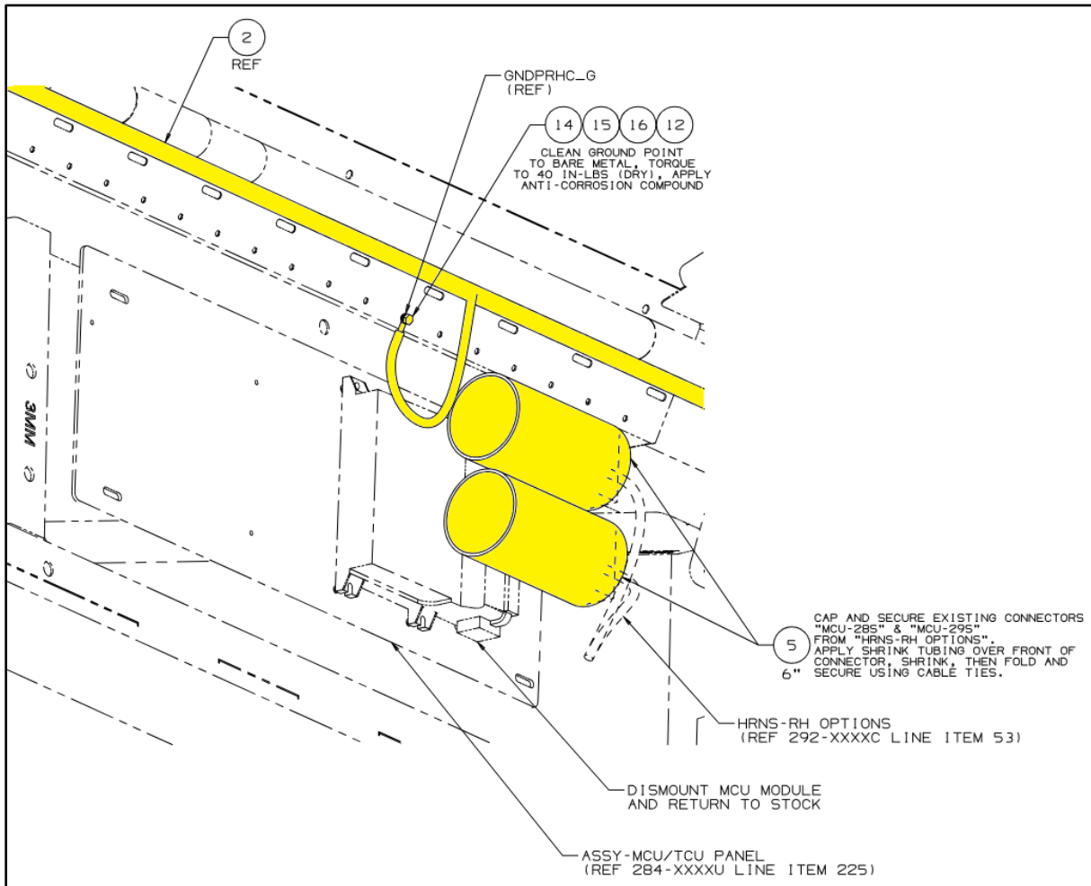
Figure 55: MCU Module Location Ref
