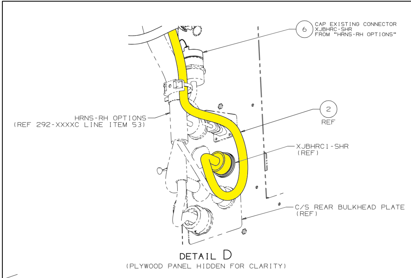
Figure 58: XJBHRC1-SHR to Plywood Panel Routing
