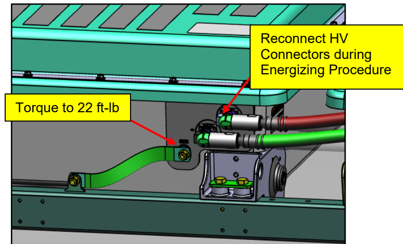
Figure 71: Upper ESS Assembly Ground Stud and HV Cable Re-installation
