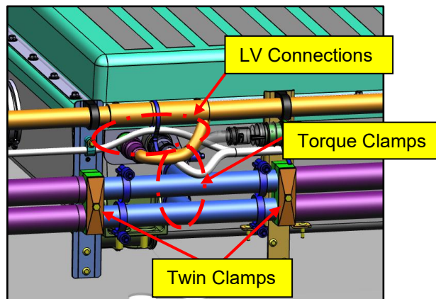
Figure 76: Upper ESS Assembly Installation Location Reference
