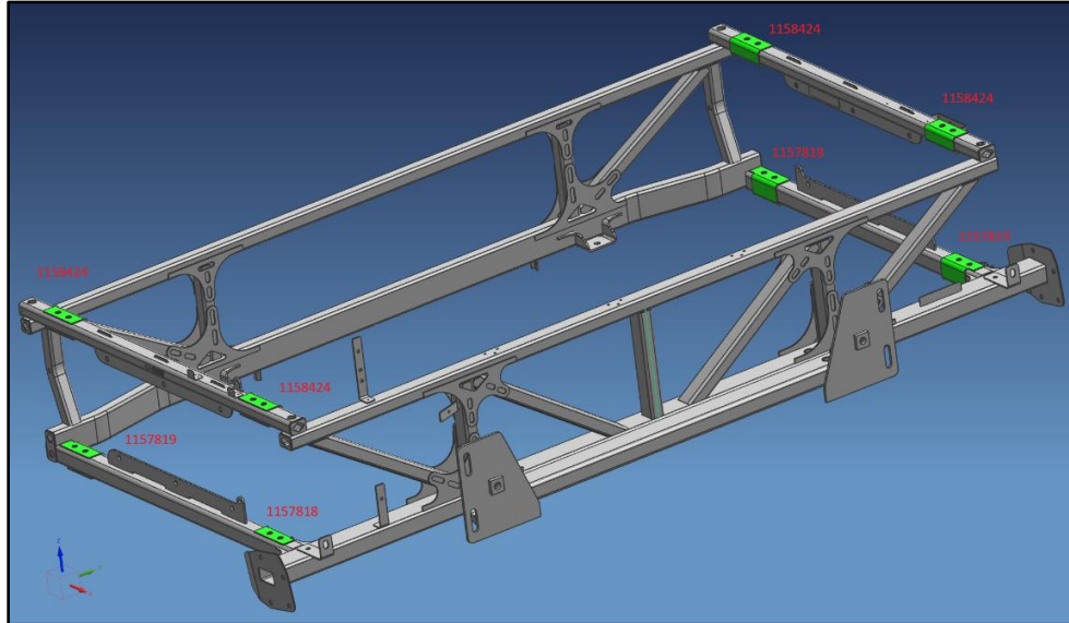
Figure 82: Reinforcement Brackets Added on Existing Rear Rack
