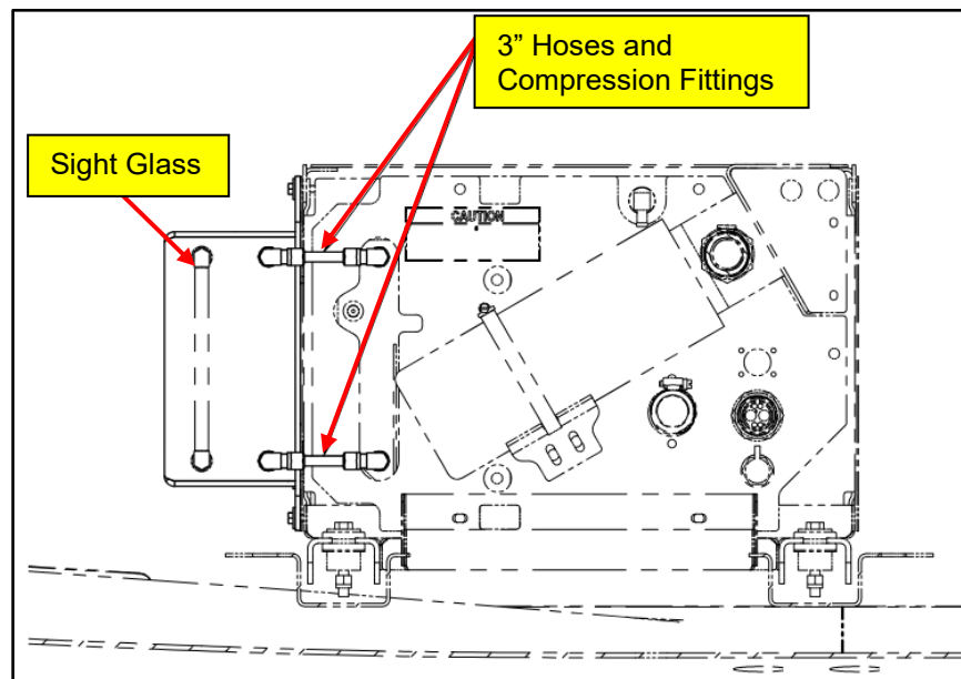
Figure 47: Sight Glass Relocation and Plumbing of BTMS Rework Reference
