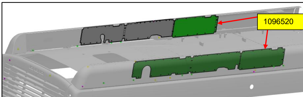
Figure 39: Added Streetside and Curbside Sidescreen Panels
