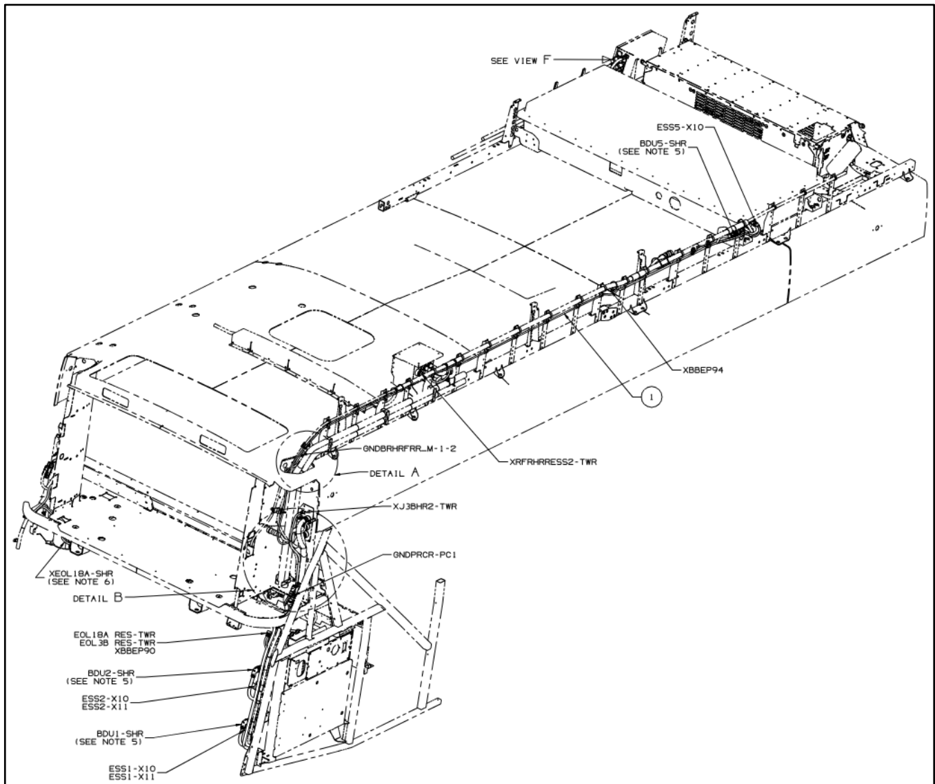
Figure 66: Rear Rooftop Jumper Harness Routing Reference
