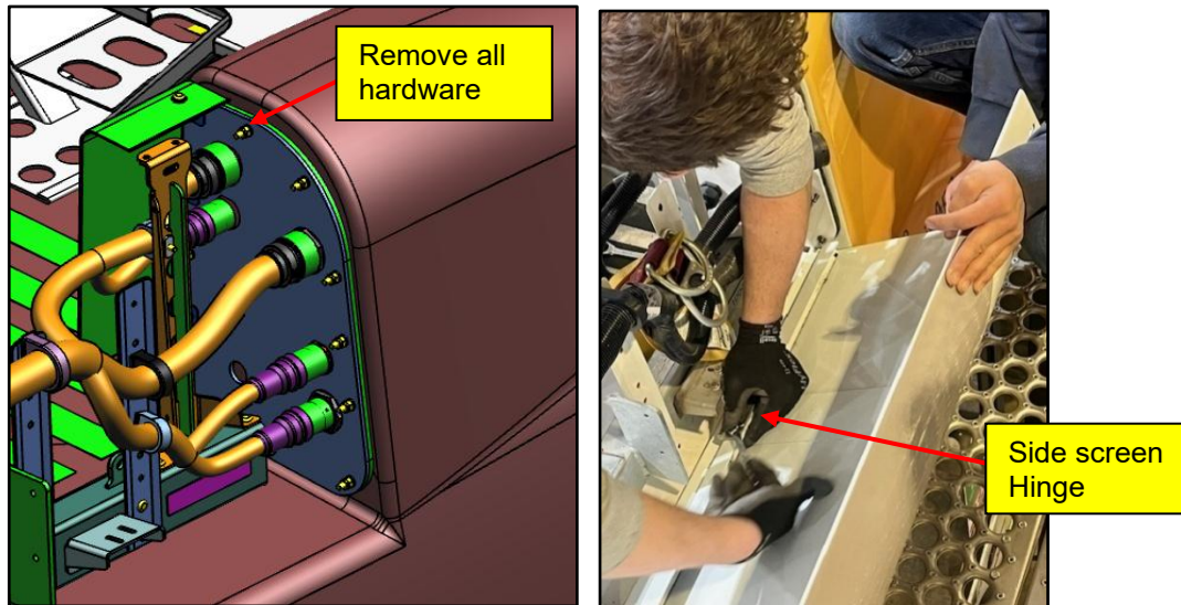
Figure 48a & 48b: Curbside Pothead Plate Removal
