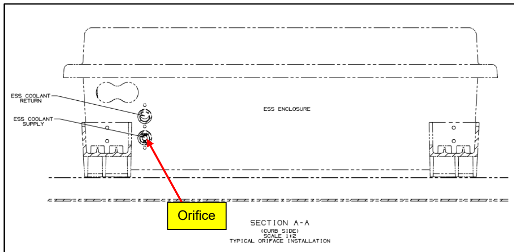
Figure 75: Orifice on ESS Coolant Supply (Lower Port)
