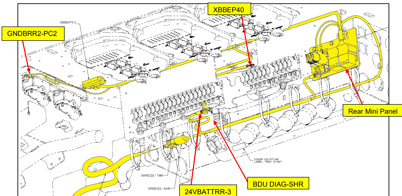
Figure 62: Rear PLC Enclosure Harness Rework
