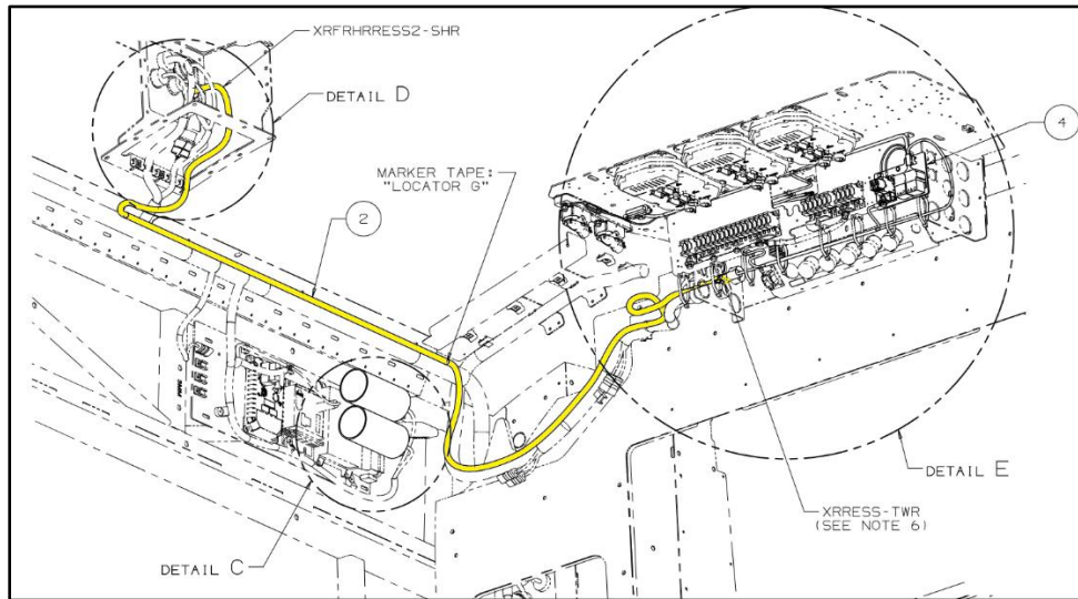
Figure 60: Jumper Harness Routing from Rear Pothead to Rear PLC Panel
