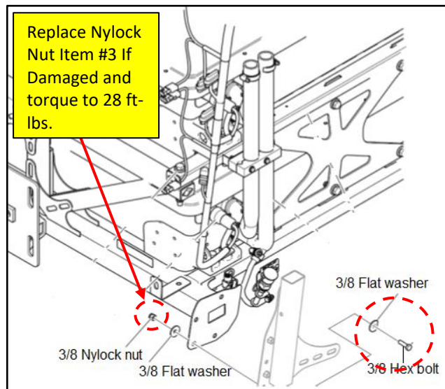
Figure 87a & 87b: ESS Ground Strap to Bus Frame and Corner Pillar Brackets to Pillar Location Reference
