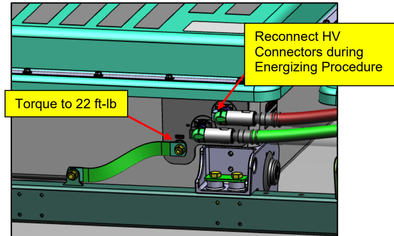
Figure 77: Upper ESS Assembly Ground Stud and HV Cable Re-installation
