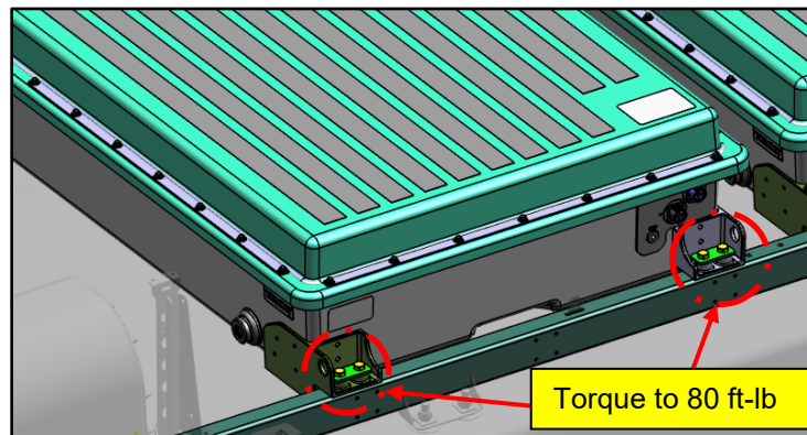
Figure 73: Upper ESS Assembly Installation Location Reference
