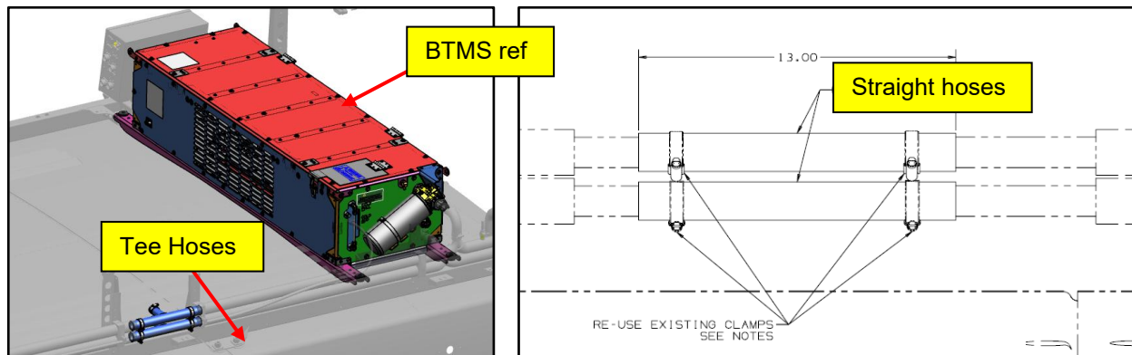
Figure 37: Coolant Hoses Replacement of Removed ESS Pack
