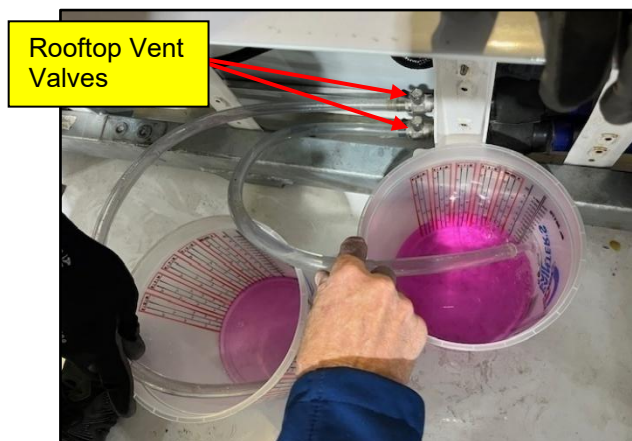
Figure 42: Drain/Flush from Rooftop Vent Valves
