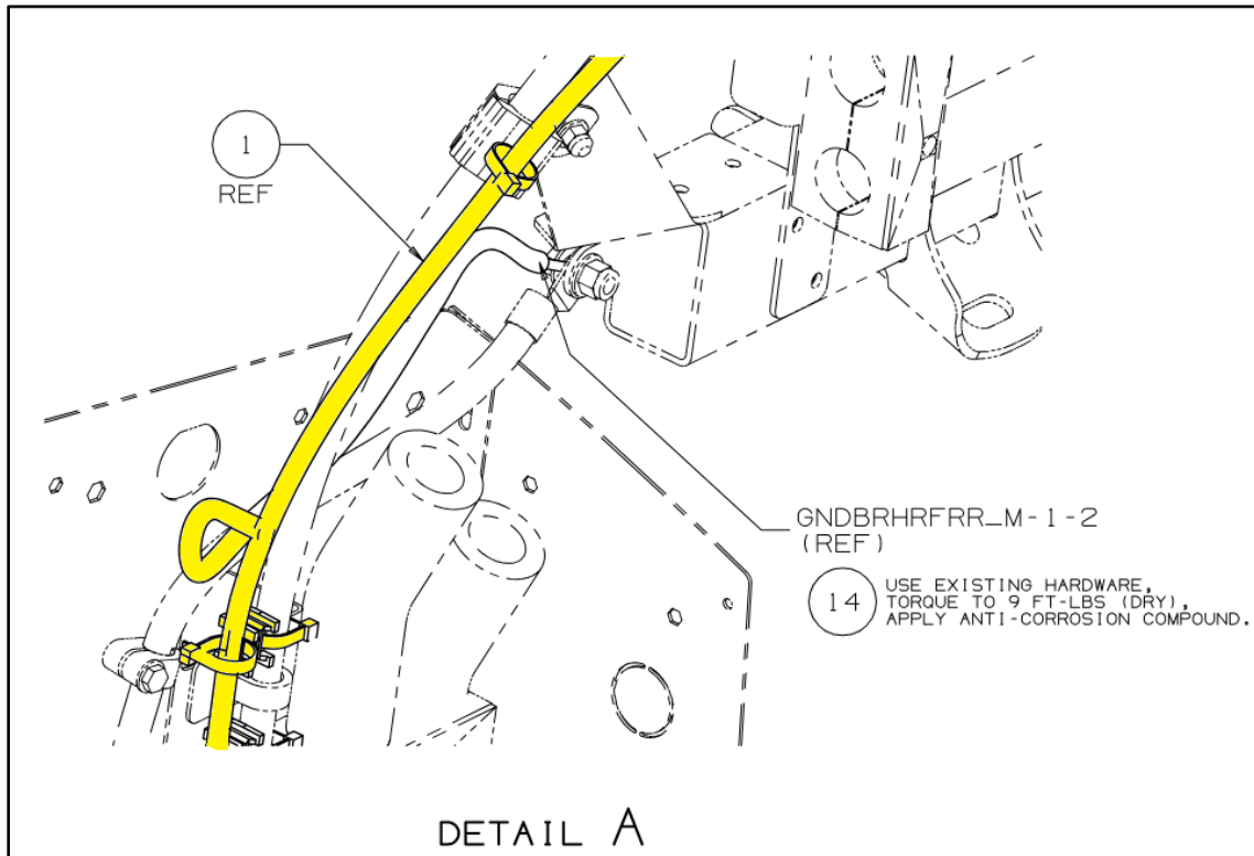
Figure 70: Ground Connection Rear Rooftop Waterfall Area
