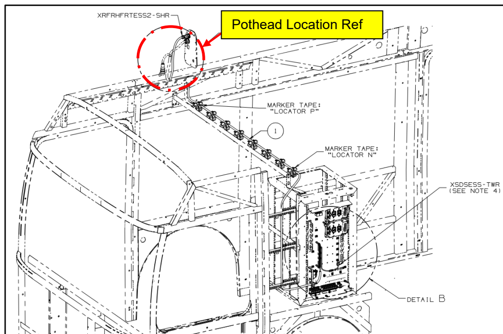
Figure 51: Jumper Harness PN 1147724 Routing Ref
