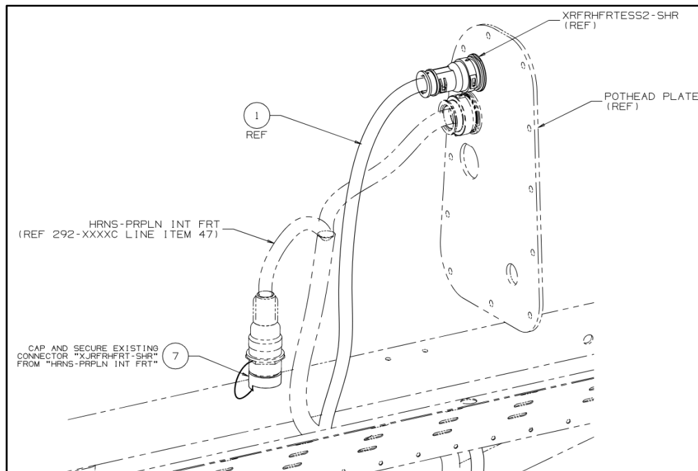
Figure 49: Front Curbside Pothead Interior Side
