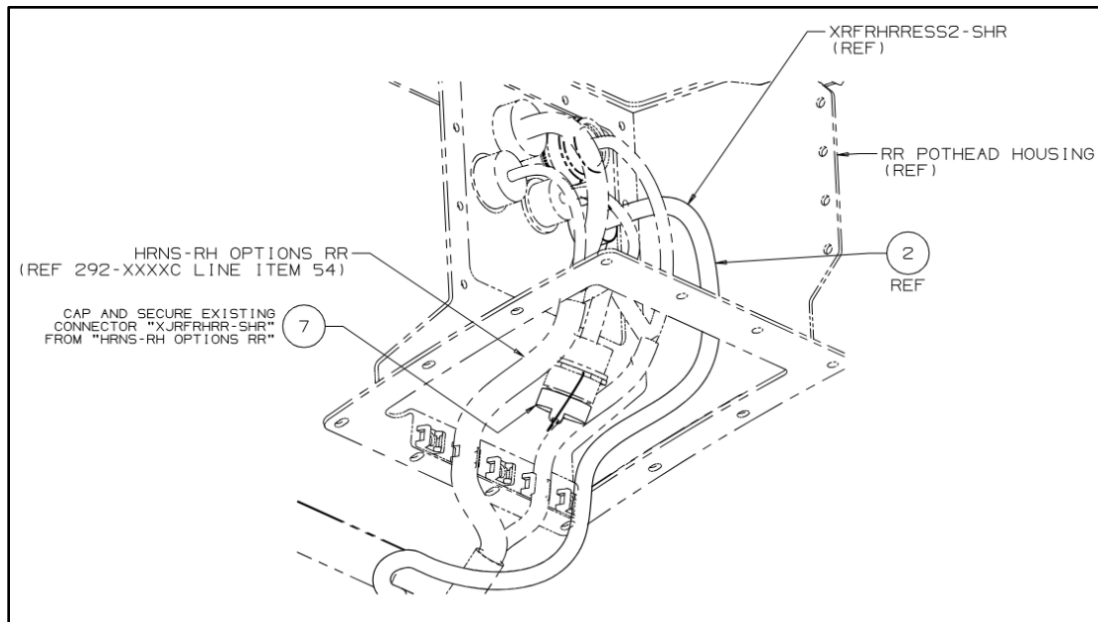
Figure 59: Rear Curbside Pothead Plate Interior Side
