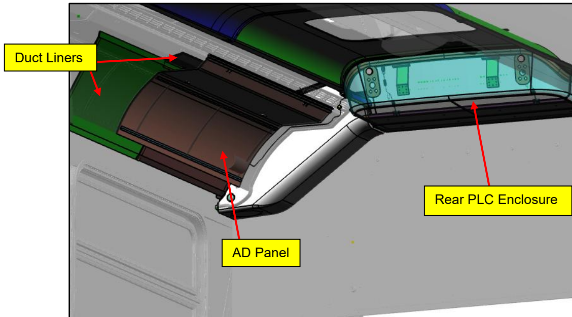
Figure 56: Rear PLC Enclosure, AD Panels and Duct Liners Reference
