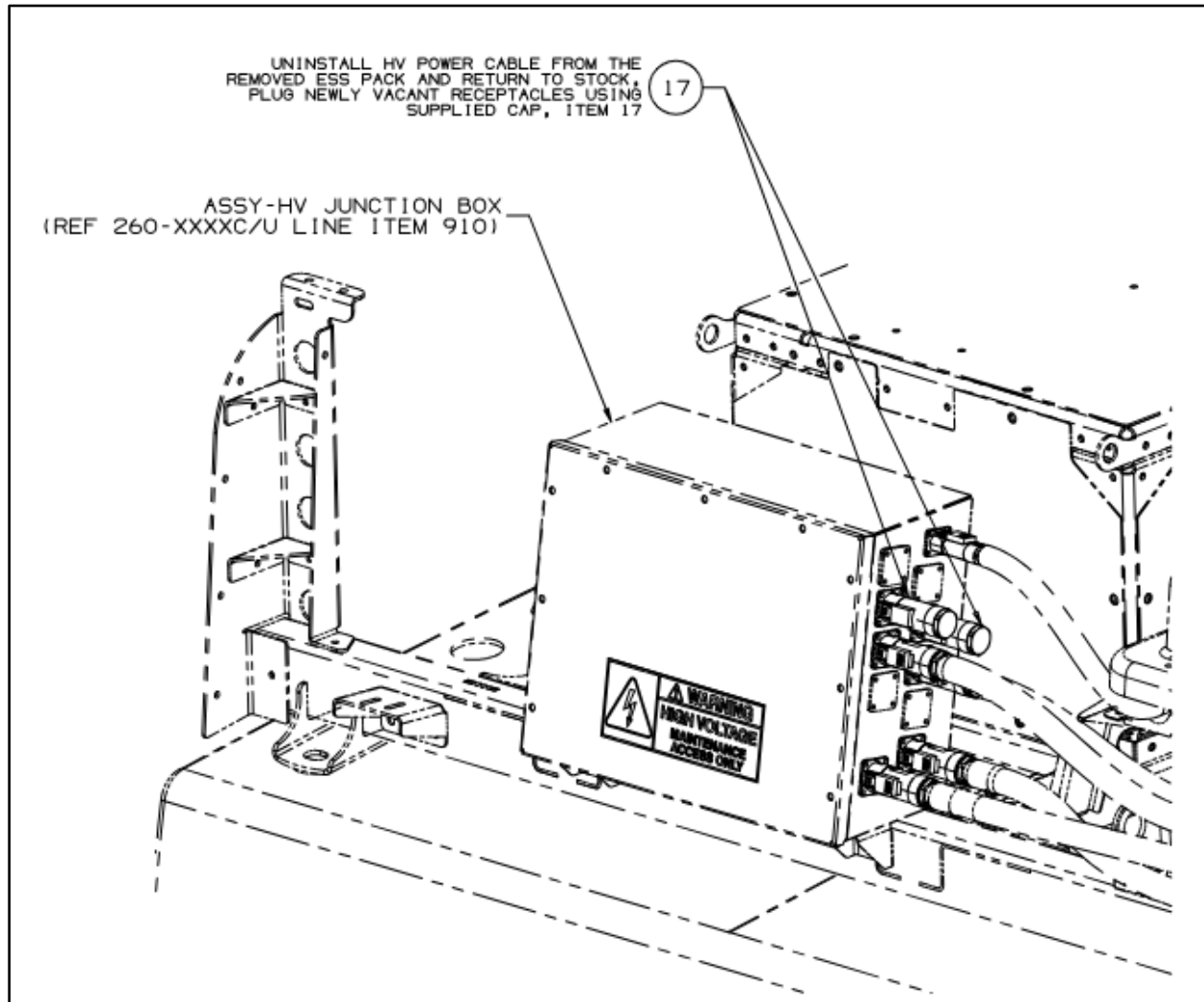
Figure 68: Roof Top HV Junction Box
