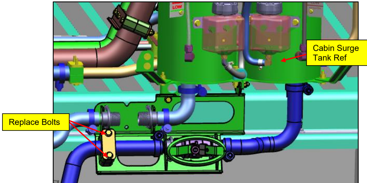
Figure 80: Coolant Hose Clamp under Cabin Surge Tank
