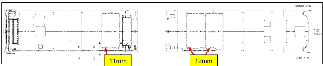
Figure 74: Orifice on ESS String # Reference
