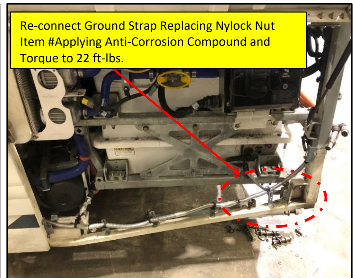
Figure 87a & 87b: ESS Ground Strap to Bus Frame and Corner Pillar Brackets to Pillar Location Reference
