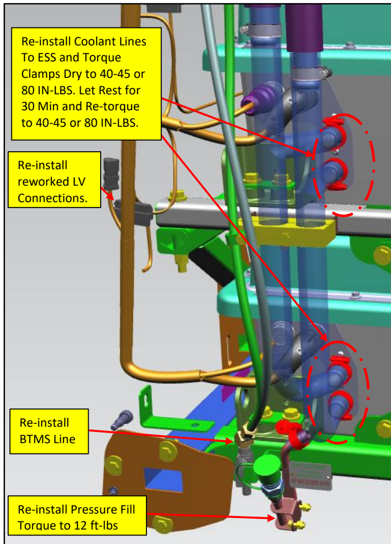
Figure 89: Low Voltage and Coolant Line Connections Location Reference
