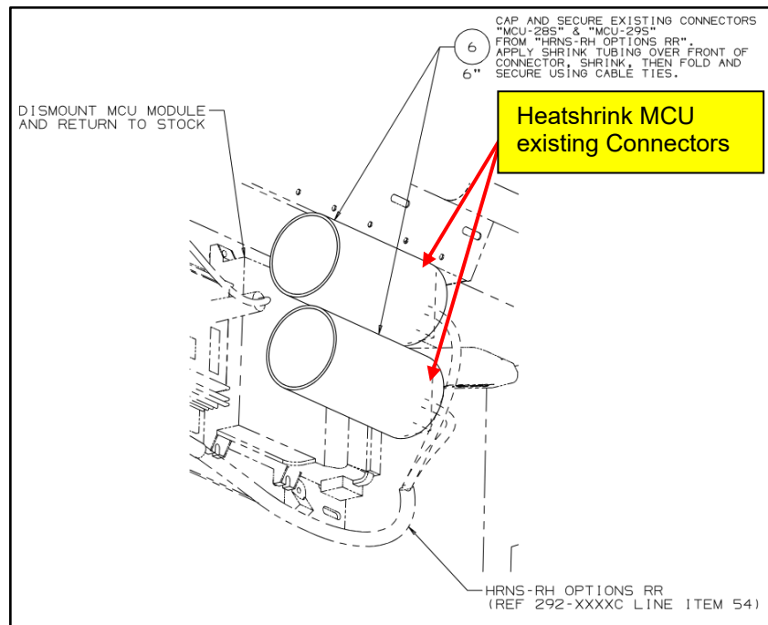
Figure 57: MCU TCU Harness Rework
