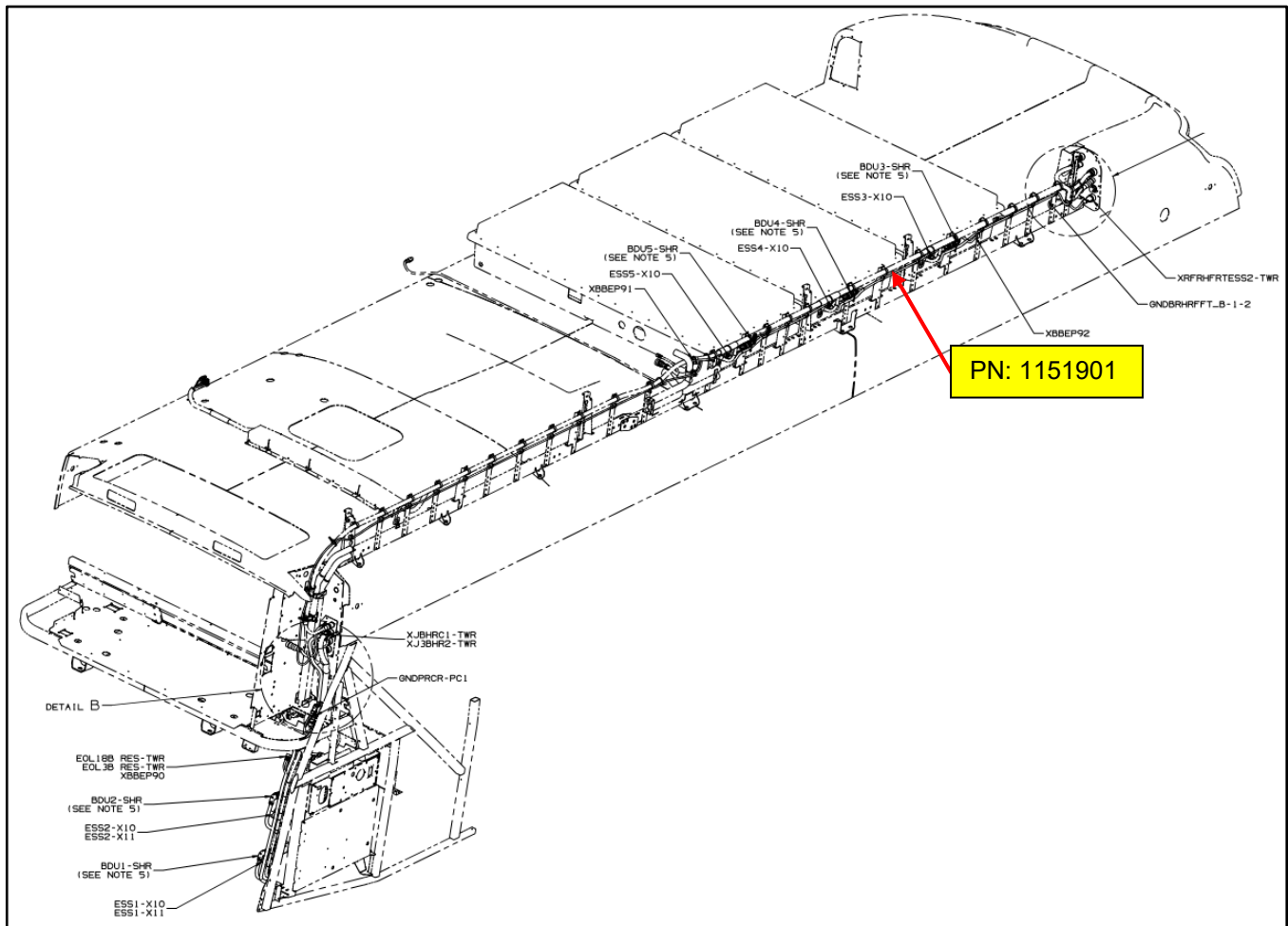
Figure 59: Roof Jumper Harness Routing Reference
