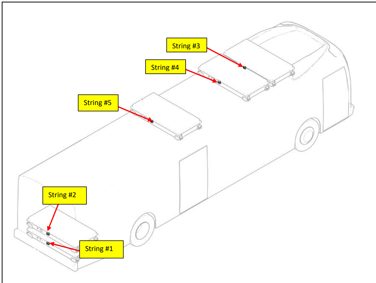
Figure 90: String Location # Reference
