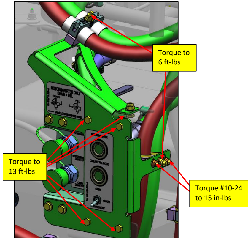
Figure 85: Cabin and Motor/Inverter Fill Panel Reinstallation
