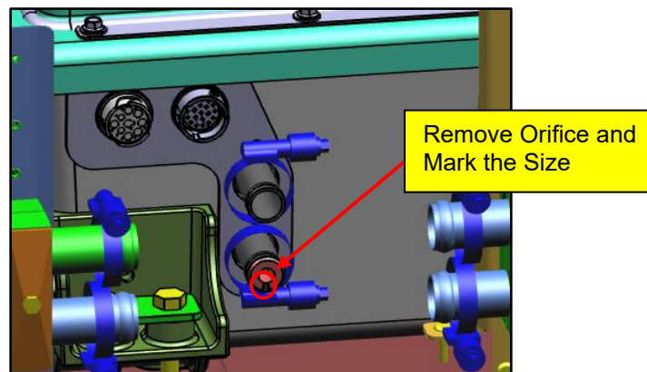
Figure 32: Reducer Orifice on ESS Pack Supply Coolant Port
