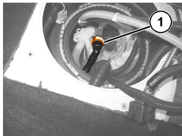
Figure 7 – Separator Coupling
