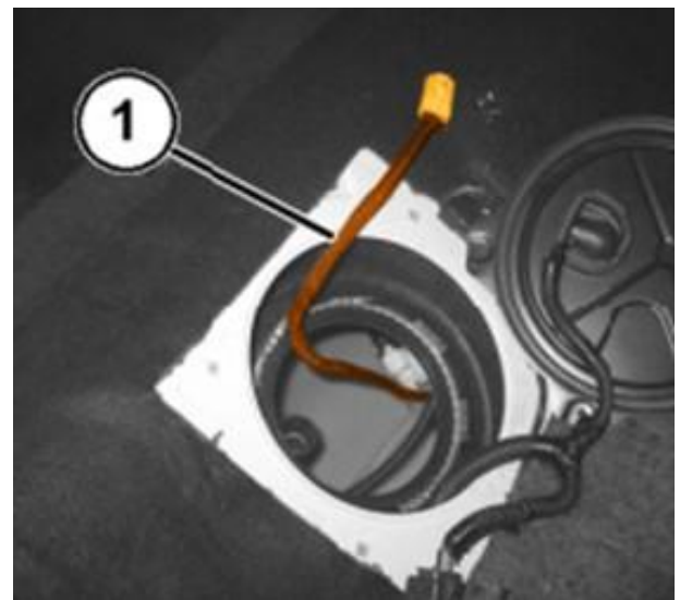
Figure 15 – Level Sensor Wiring
