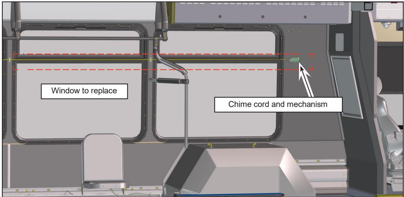
Figure 2 - Remove the Chime Cord That is Preventing the Window From Being Removed (Some Parts Omitted for Clarity, Your Configuration May Differ)
