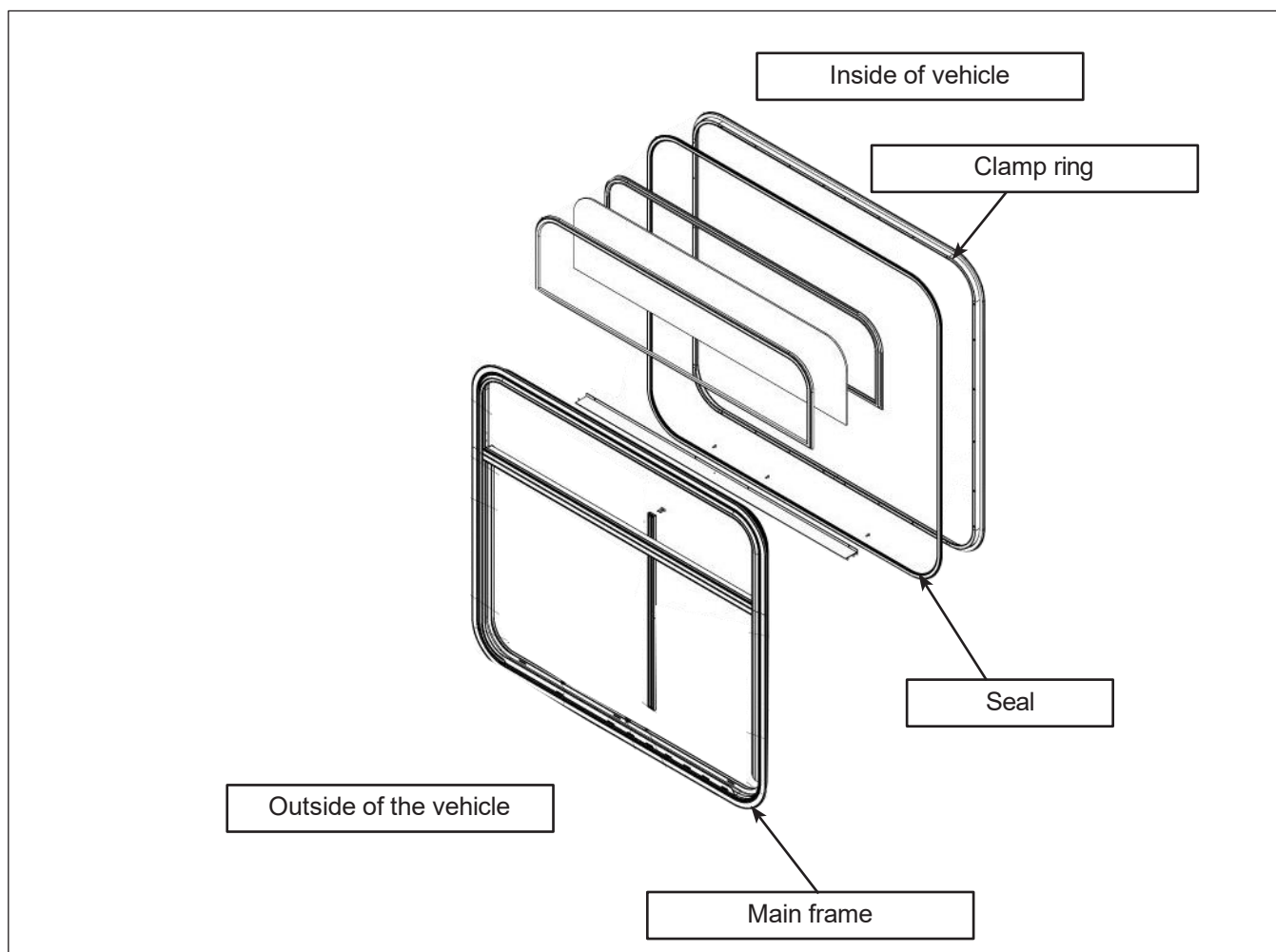
Figure 14 - Typical Example of Window Components
