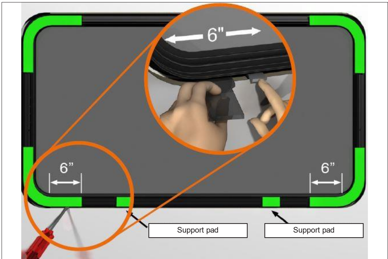
Figure 20 - Use a Lever or Install Shims Only in the Areas Indicated in Green
