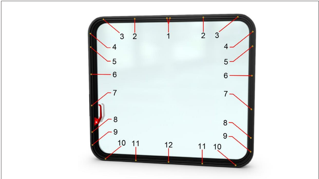
Figure 22 - Screws Torque Sequence
