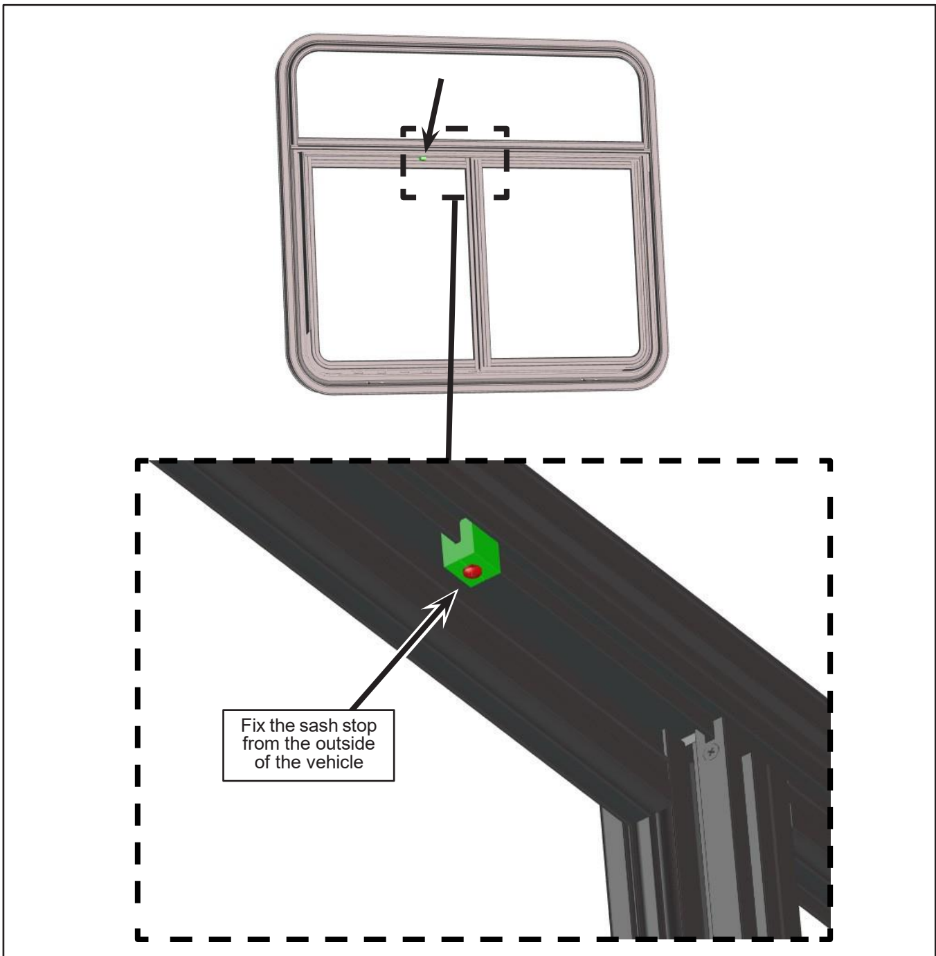
Figure 24 - Install a Sash Stop
