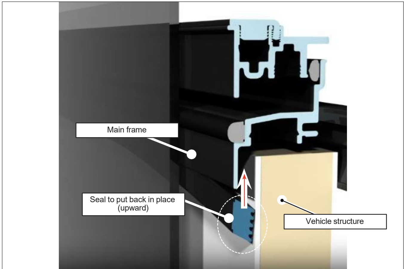
Figure 19 - Put the Seal Back in Place if Required
