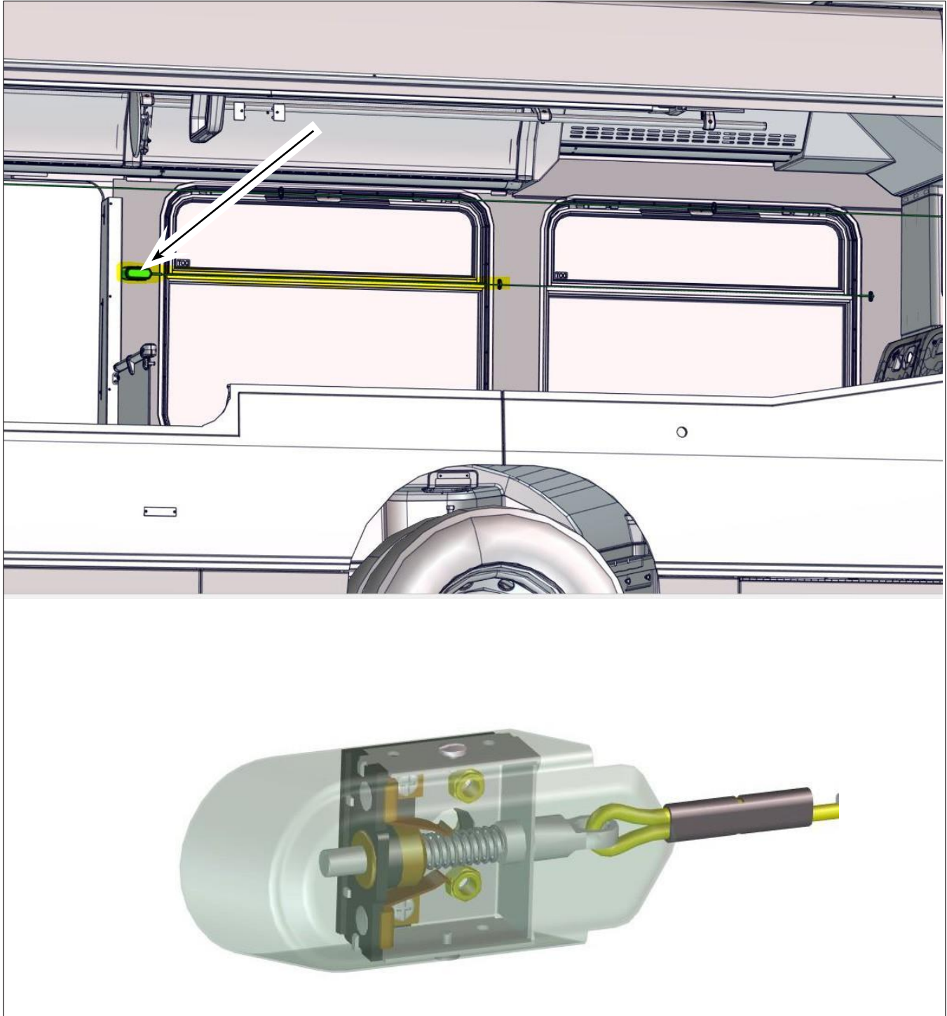
Figure 13 - Remove the Chime Cord (Your Configuration May Differ)
