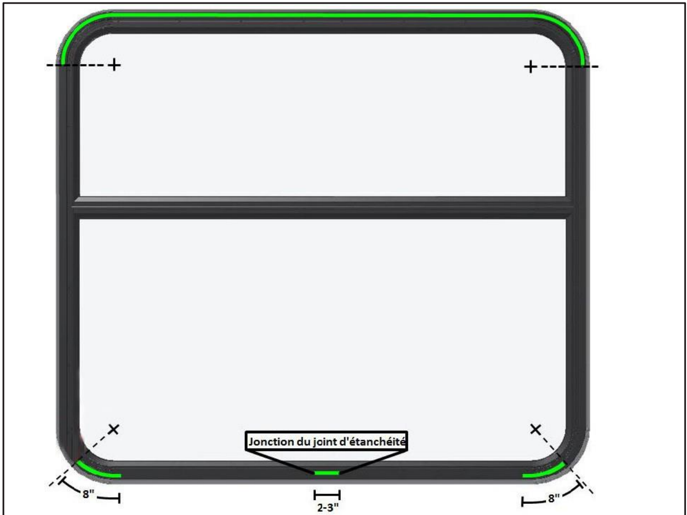
Figure 18 - Apply Butyl to the Body Seams
