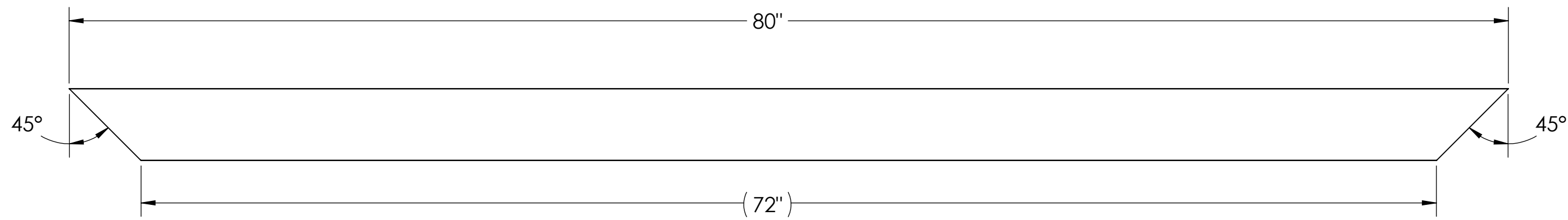
SIDE VIEW
