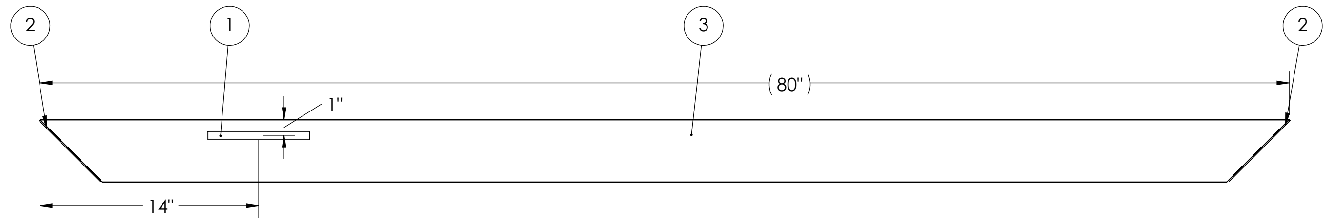
SIDE VIEW
