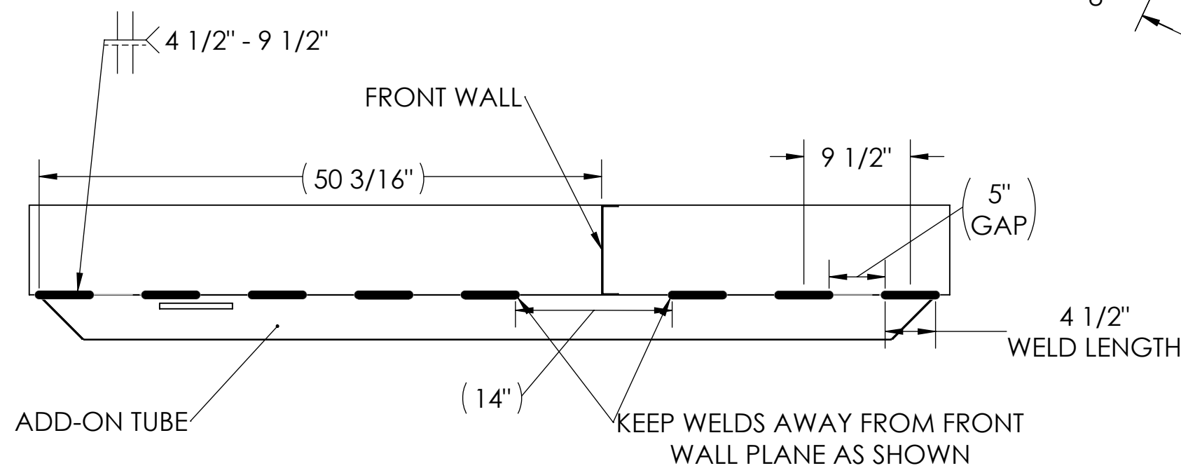
SIDE VIEW - WELD LENGTH AND GAP
