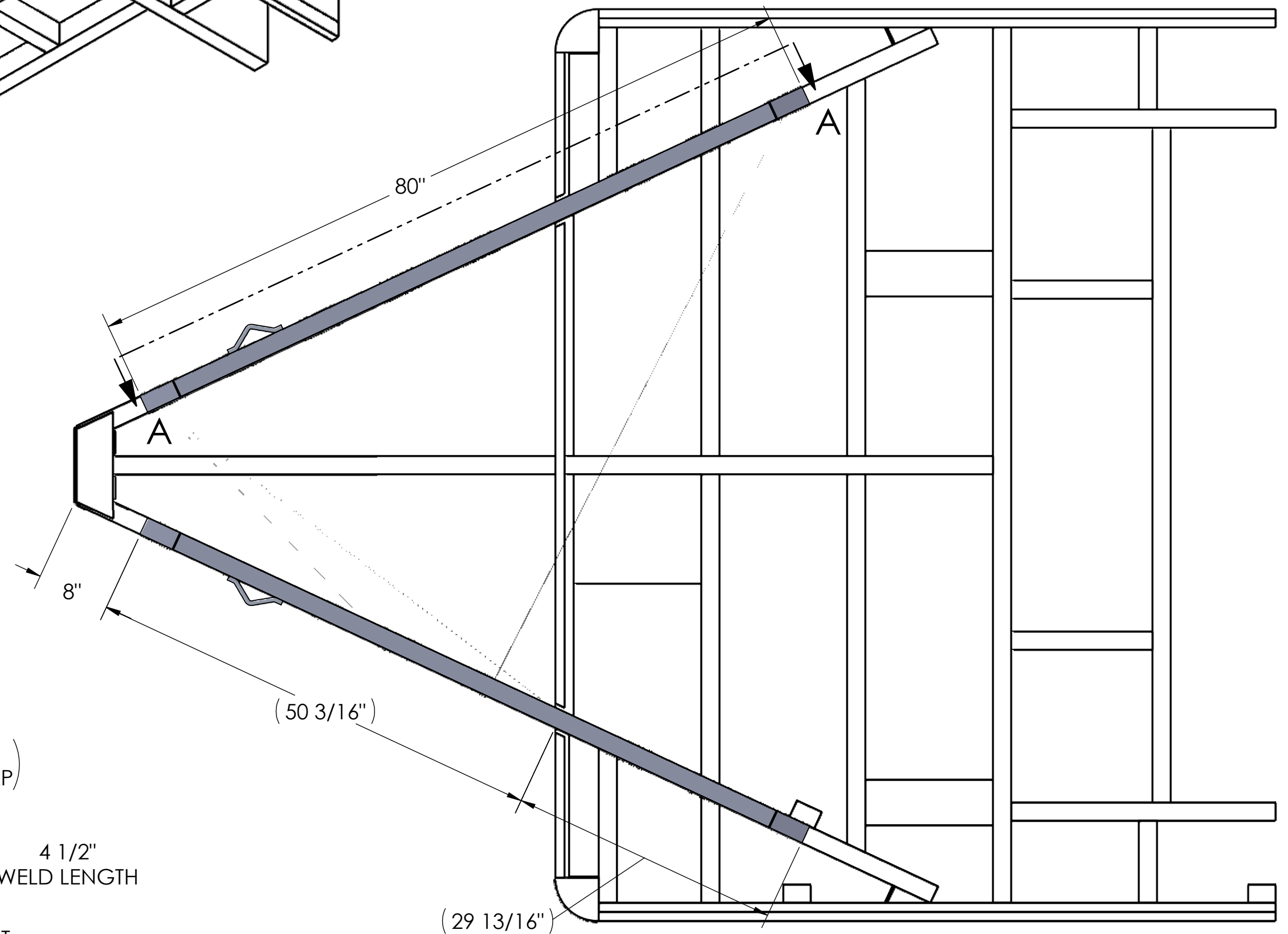
BOTTOM VIEW
