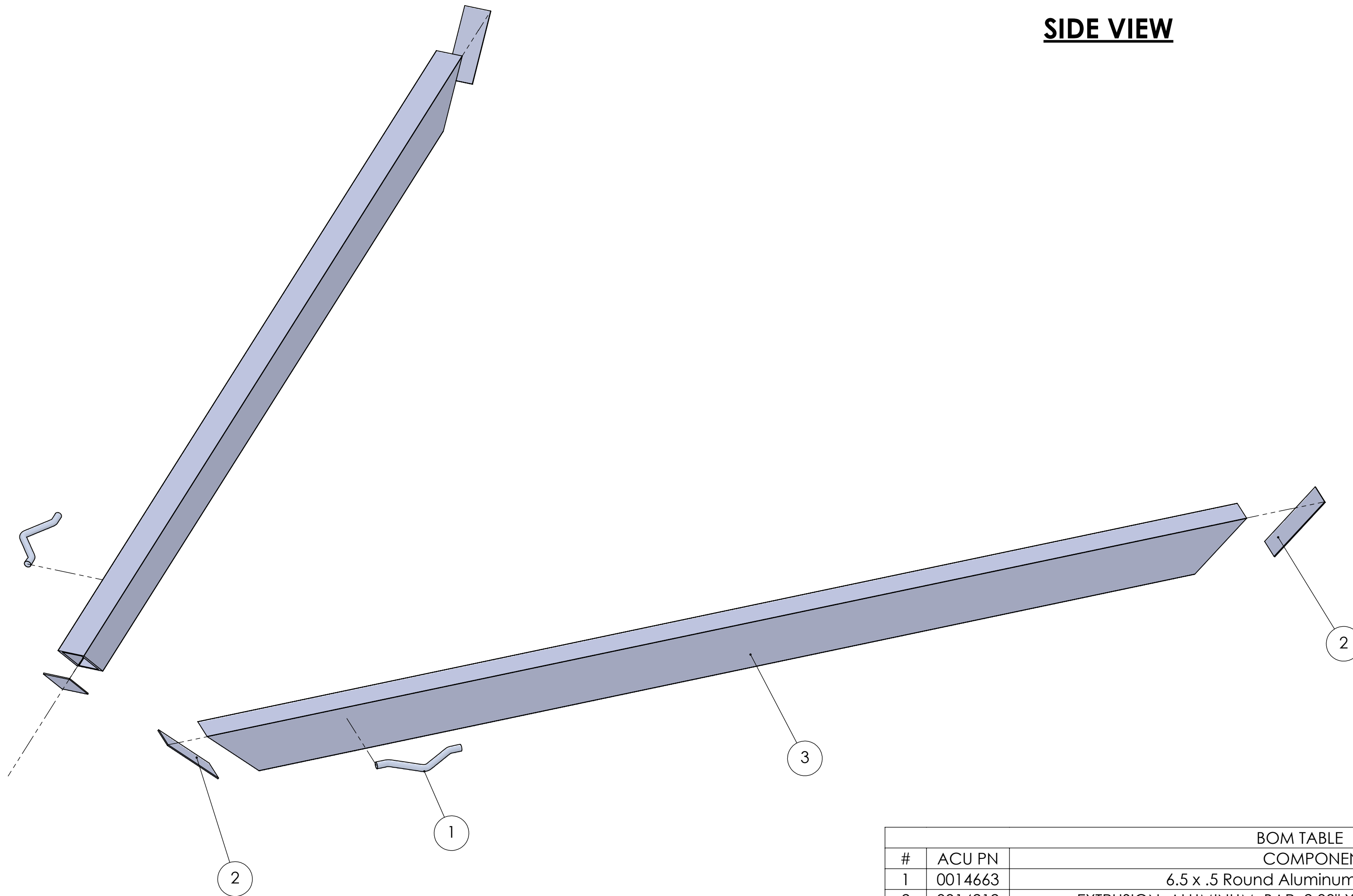
ISO EXPLODED VIEW
