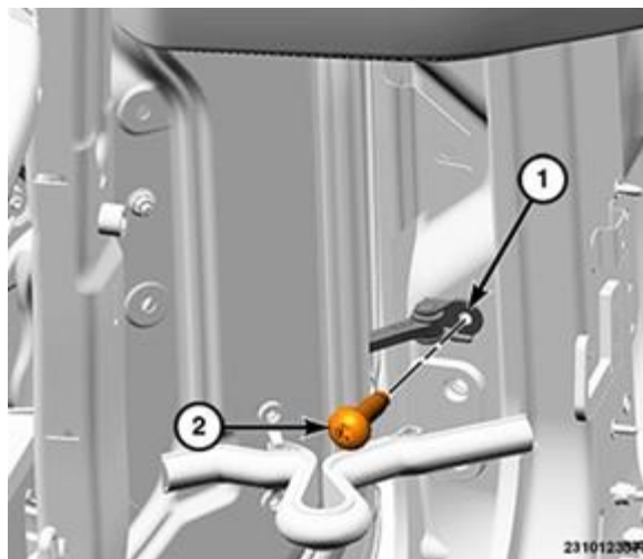
Figure 15 – Door Check Bolt
