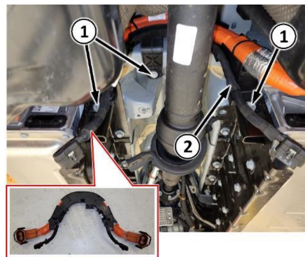
Figure 51 – HV Battery Jumper Harness
