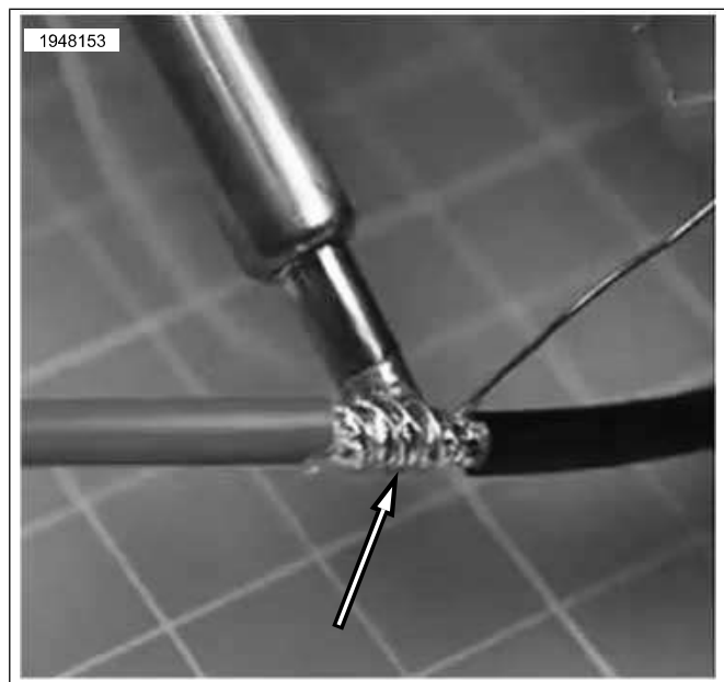
Figure 20. Add and Melt Solder with Soldering Iron
