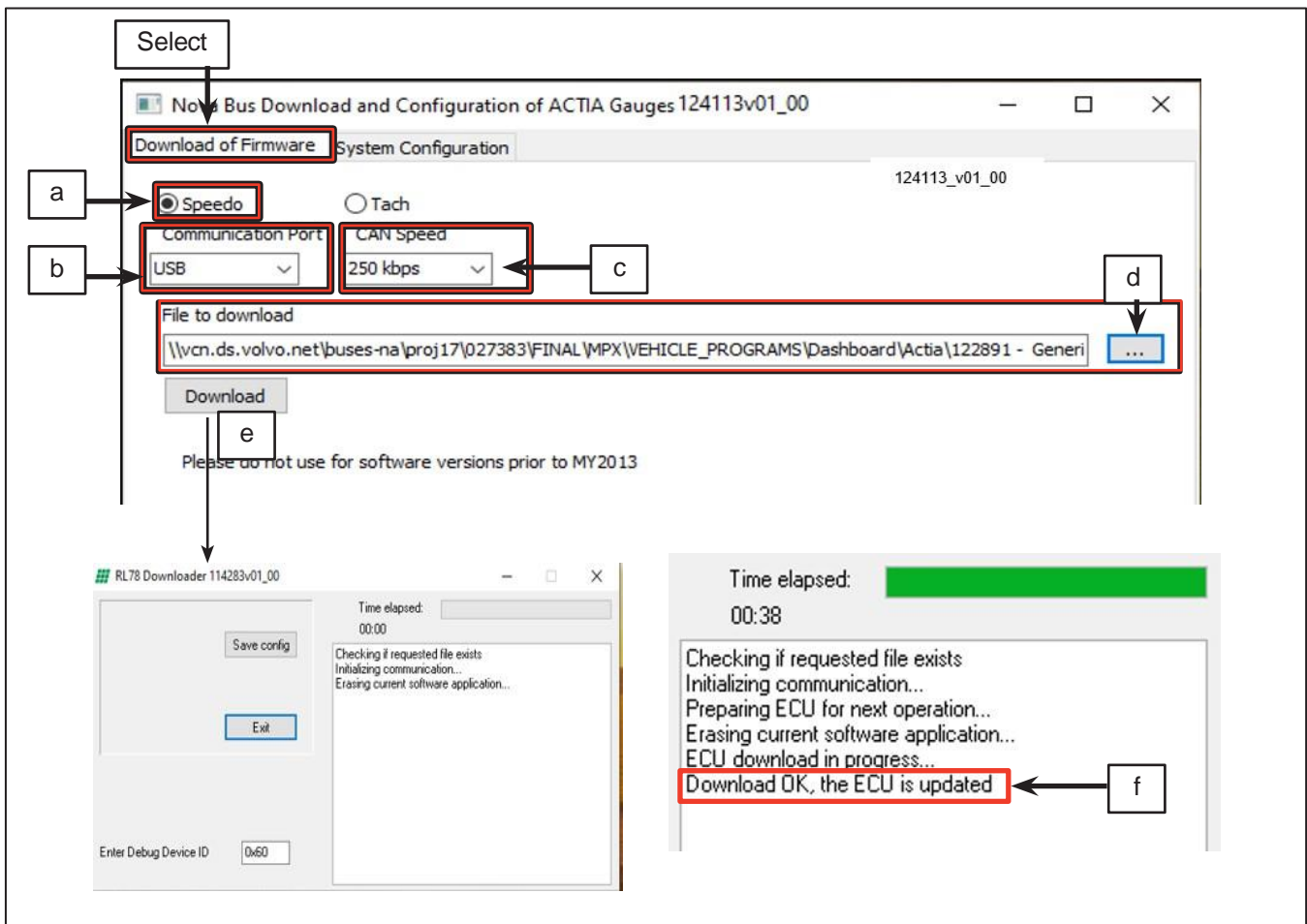
Figure 4 - New Software Download Procedure Step by Step
