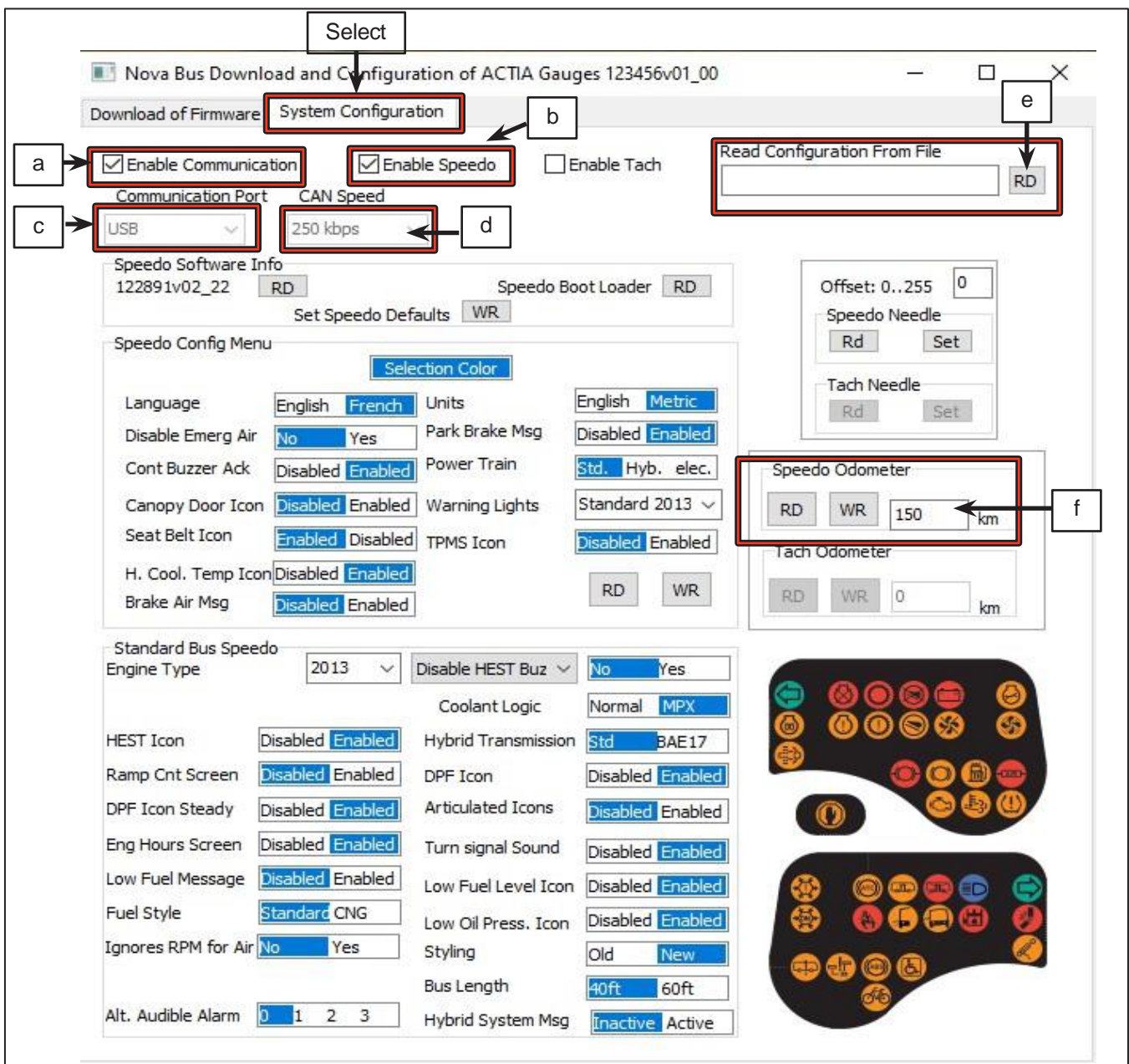
Figure 5 - Speedometer Parameter Download Step by Step
