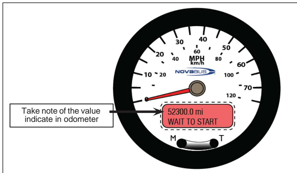
Figure 2 - Speedometer Odometer
