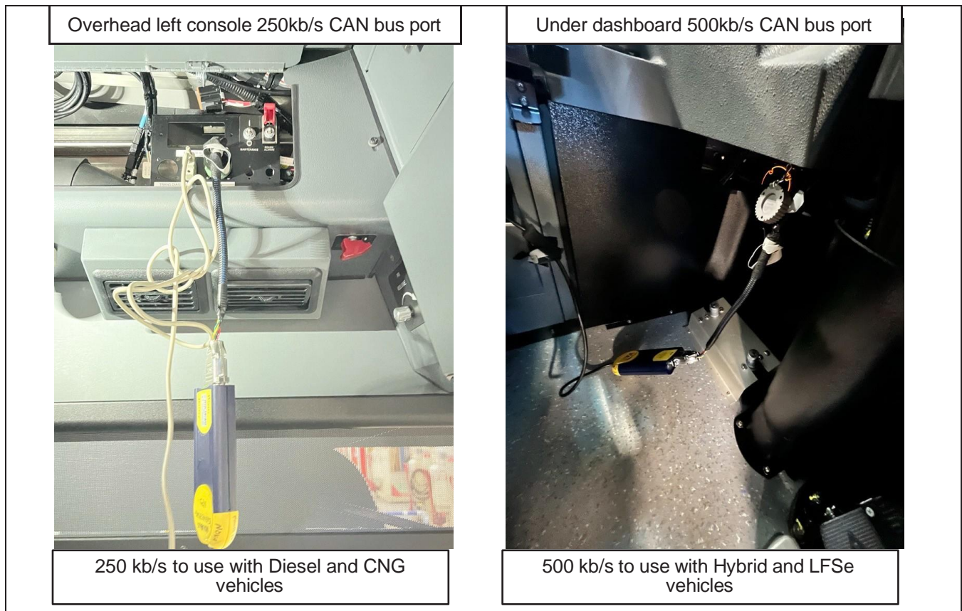
Figure 3 - DDR Port Location
