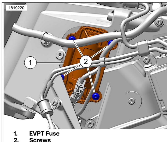
Figure 3. EVPT Fuse
