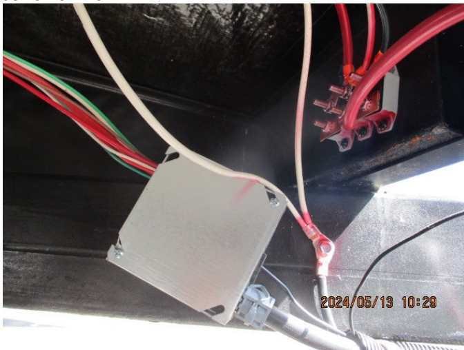
JUNCTION BOX
