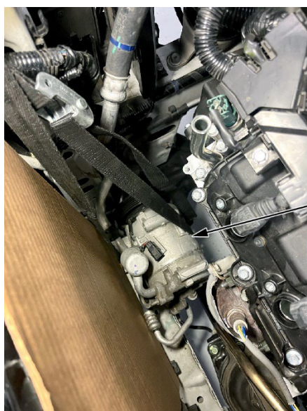
SECURED COMPRESSOR
