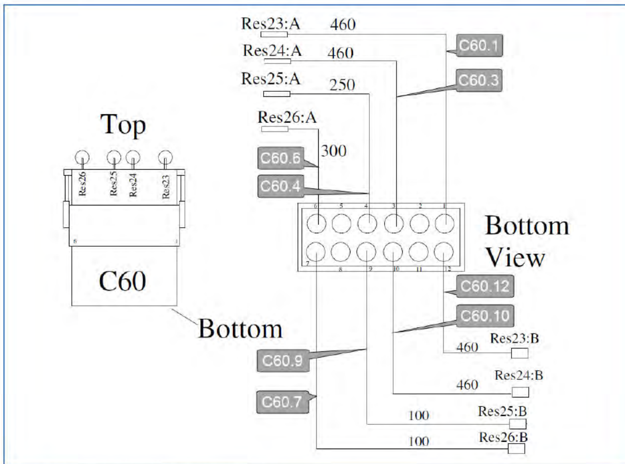
FIGURE 1: 0600179 RESISTOR HARNESS (CONNECTOR C60)
