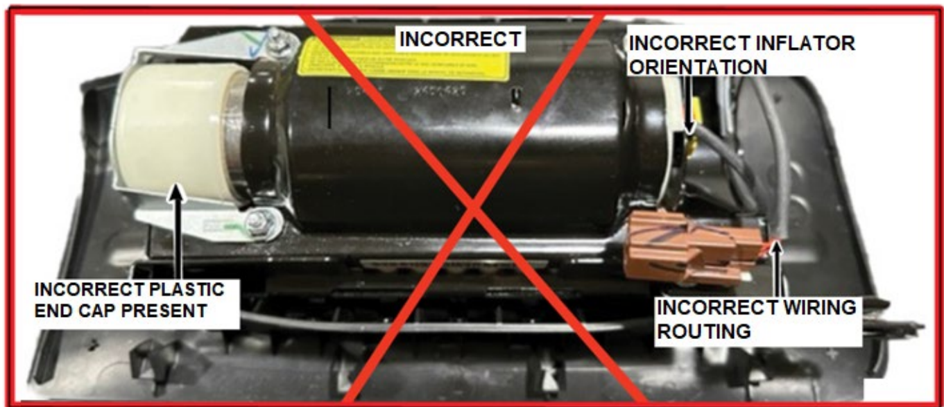
FIGURE 2 – NO GOOD (NG) INCORRECT INSTALLATION: TAKE CLEAR REQUIRED CLAIM PHOTO #1, NO GOOD INSTALLED AIR BAG SIMILAR TO BELOW. THEN CLICK HERE TO PROCEED TO STEP 8.
