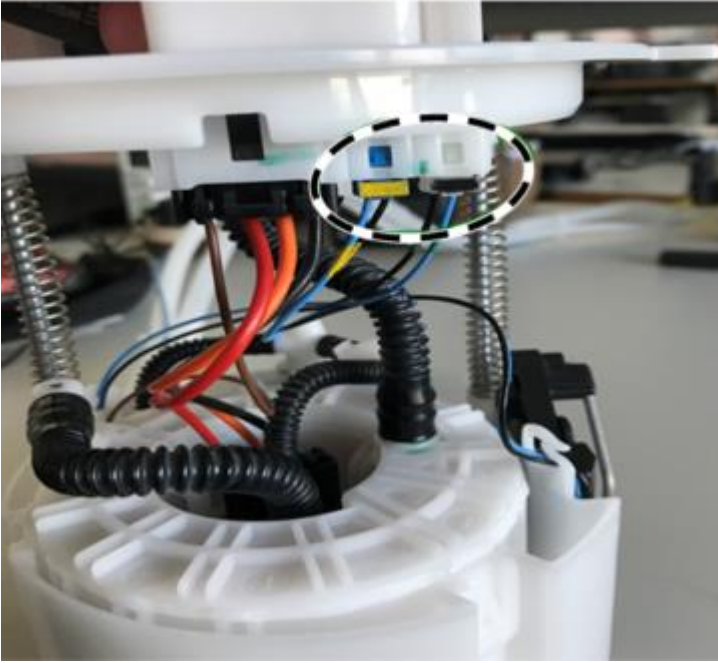
Figure 2 (release corresponding connector and disconnect the contacts)
