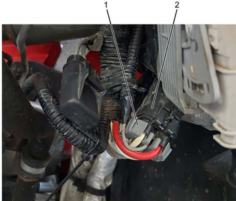
Figure 4. Booster Pump Motor Jumper Harness Connector
