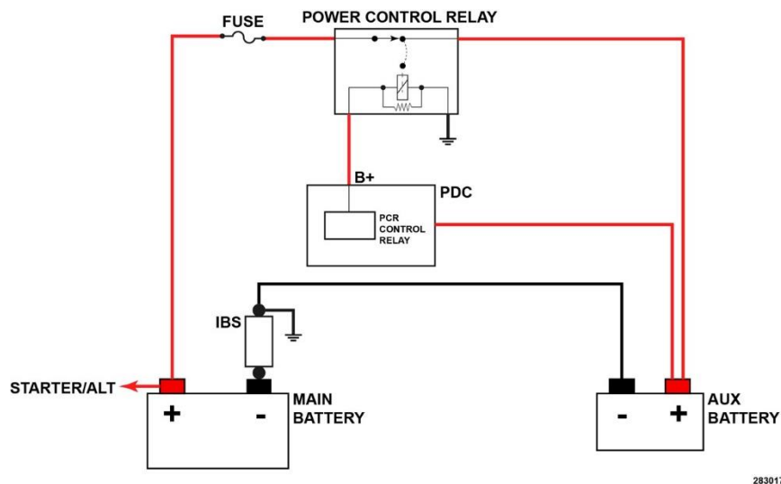
Figure 175 – Dual Battery System
