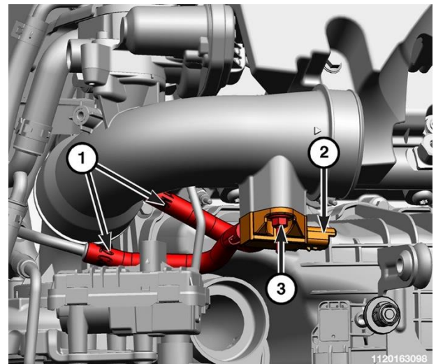
Figure 117 – Differential Pressure Sensor
