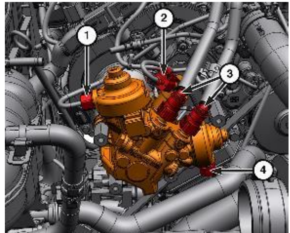
Figure 34 – HPFP Connections
