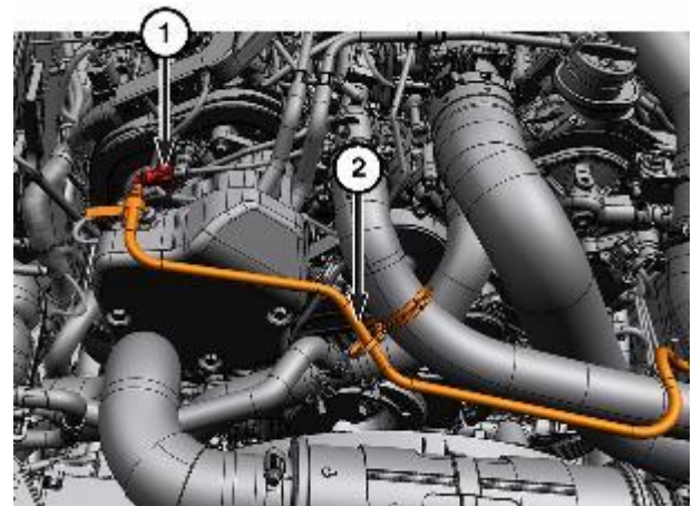
Figure 3 – Vacuum Line
