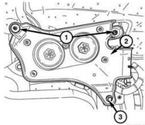
Figure 53 – Fuel Filter/Water Separator
