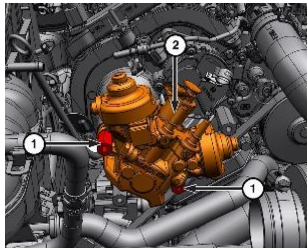
Figure 35 – Upper Bolts
