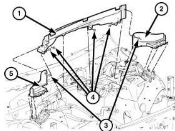
Figure 26 – Engine Cover
