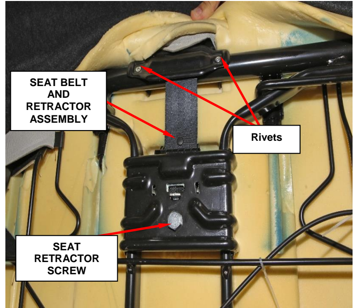
Figure 36 – Seat Back Frame
