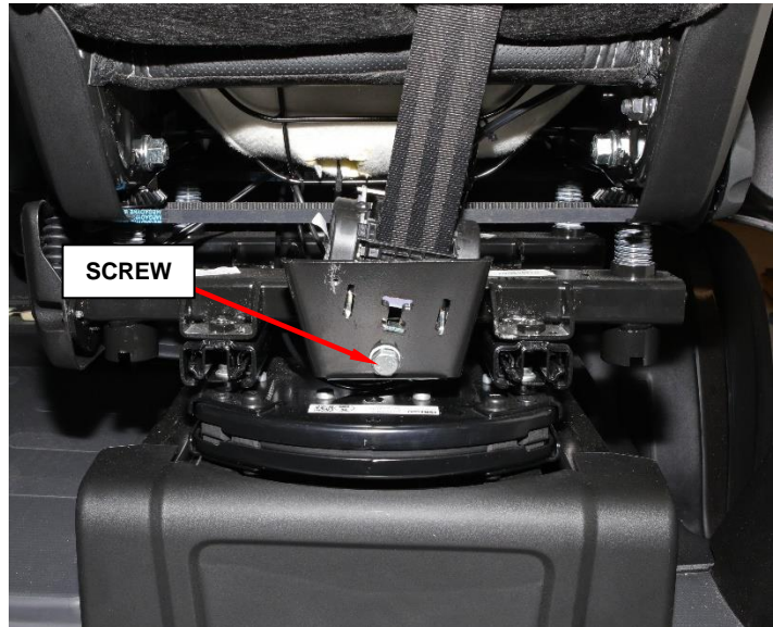
Figure 25 – Retractor Screw
