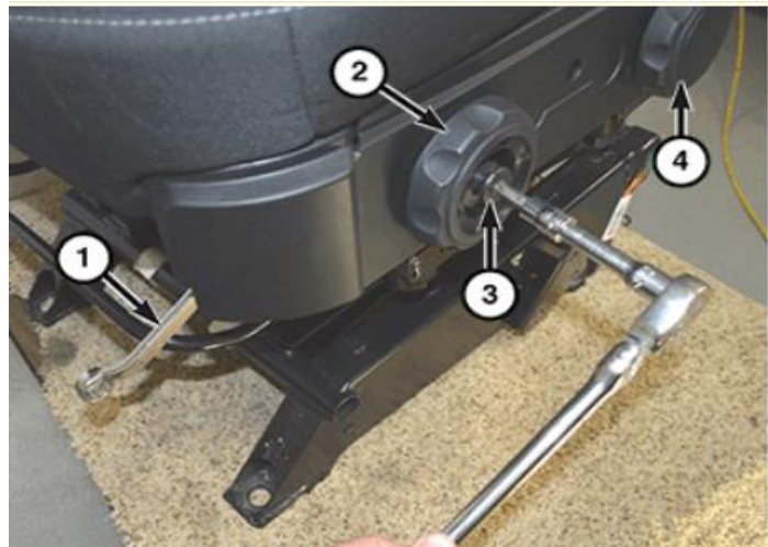
Figure 20 – Bolt Removal
