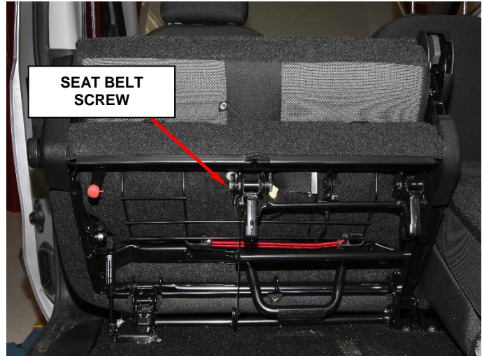
Figure 33 – Rear Seat
