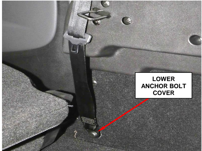
Figure 37 – Anchor Screw
