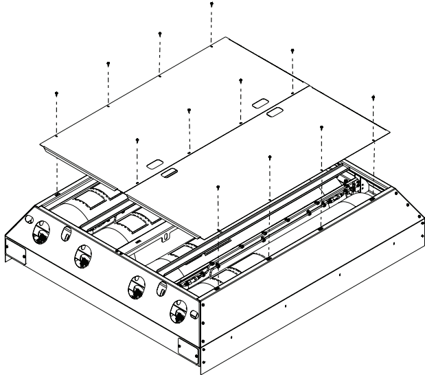
Illustration represents reinstalling all covers on the Roof Mount CNG tank configuration.
