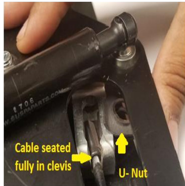
Figure 3 – Cable Seating
