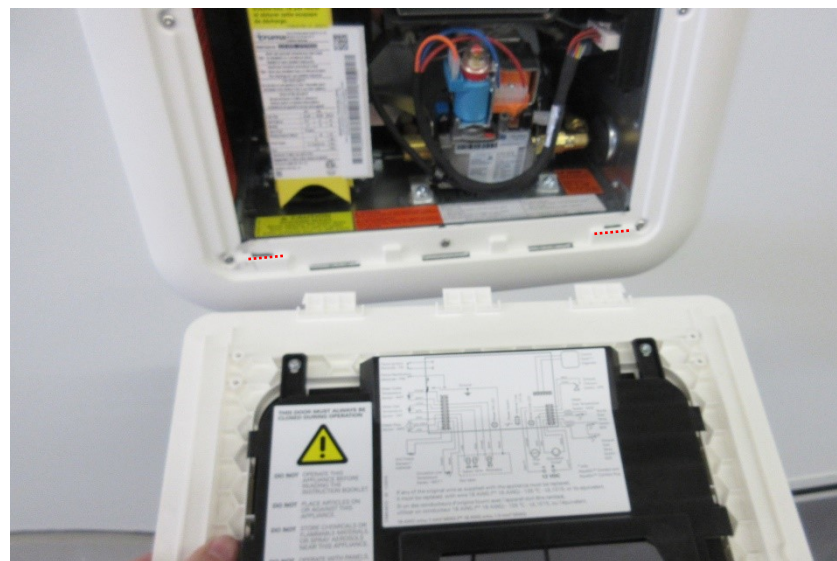
Cut each strap as close to the door frame as possible. Discard screws and straps and reinstall door.
