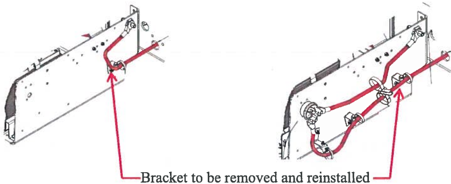
Rear Frame Battery without Battery Disconnect Switch
