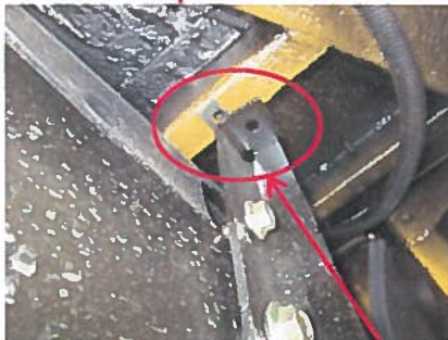
Example shown of front brace missing fasteners at floor and loose at battery box attachment.
