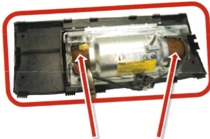
PASSENGER AIRBAG INFLATOR
