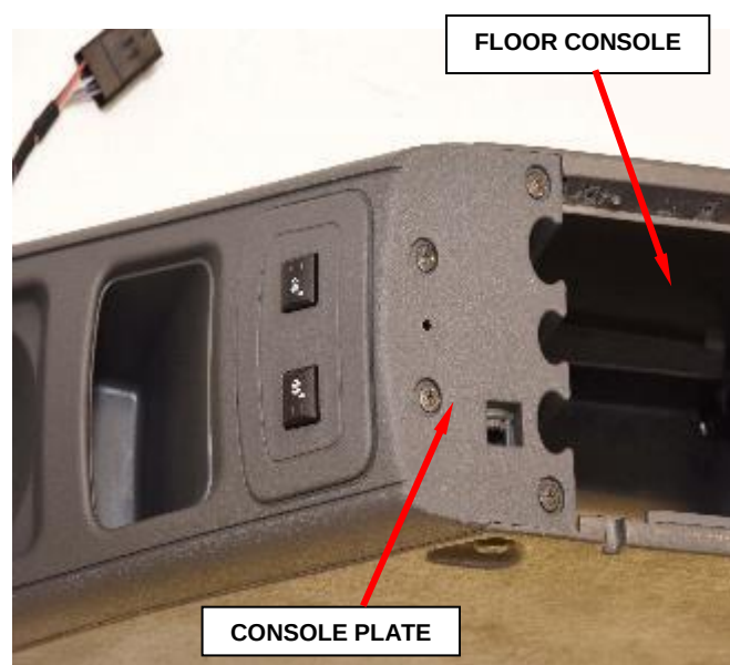
Figure 10 – Console Plate to Floor Console
