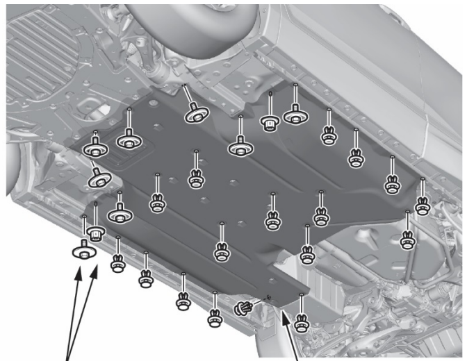
BOLTS AND NUTS 9.4 N·m (6.9 lb-in)
