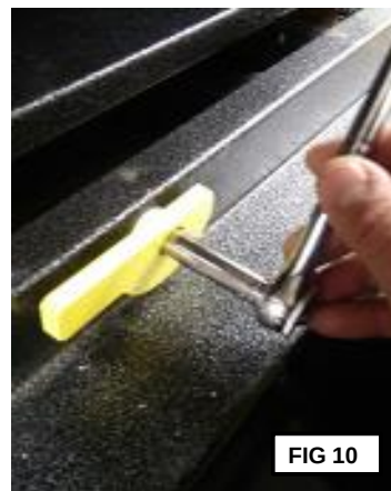
FIG 10: Tighten 1/4 turn of 10mm socket. Note: DO NOT over tighten - brass threads will strip
