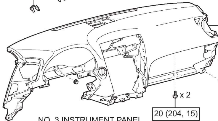
NO. 3 INSTRUMENT PANEL REGISTER ASSEMBLY
