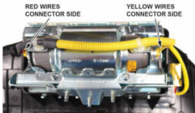
ORIGINAL INFLATOR HARNESS ROUTING
