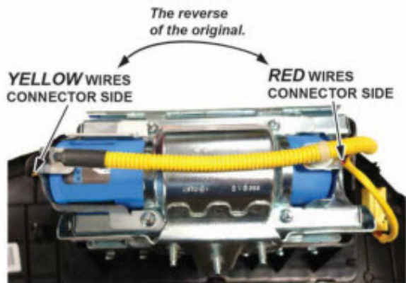
NEW INFLATOR HARNESS ROUTING
