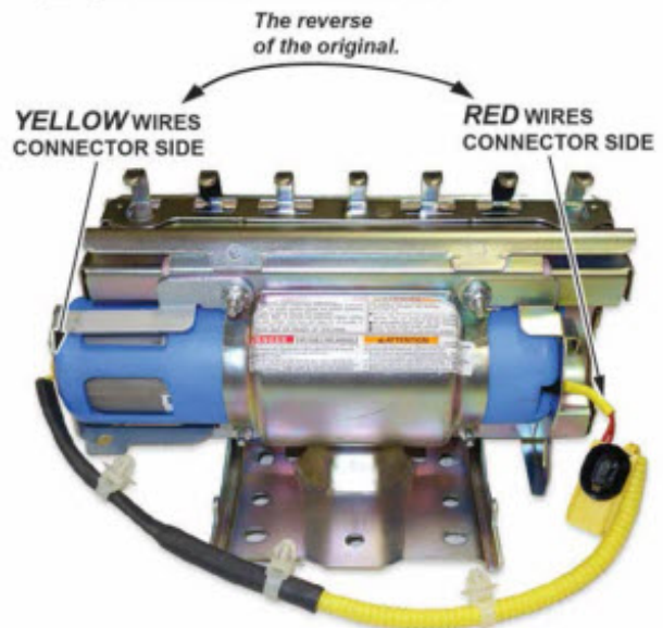
NEW INFLATOR HARNESS ROUTING
