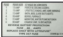
Decal, 12V Fuse Panel
