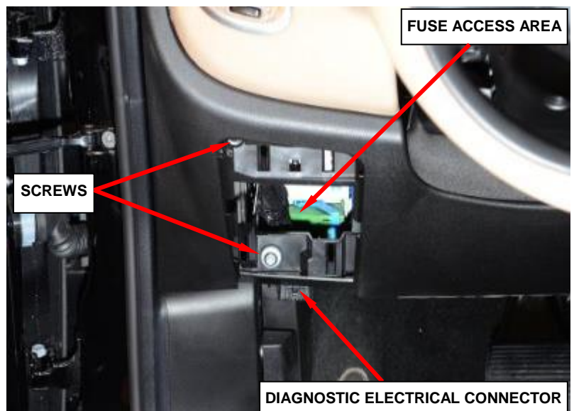
Figure 8 – Fuse Cover
