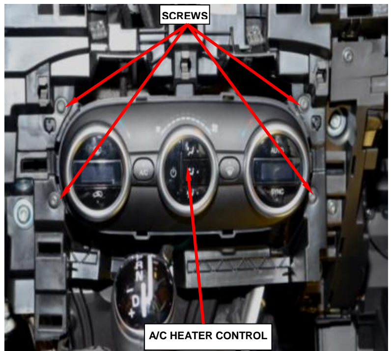
Figure 32 – HVAC Control
