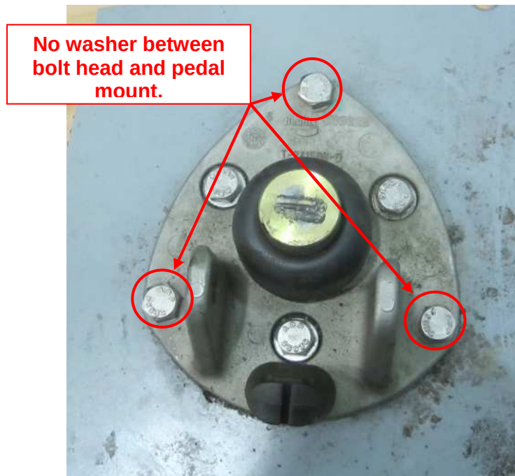
Figure 12: Pedal Mount
