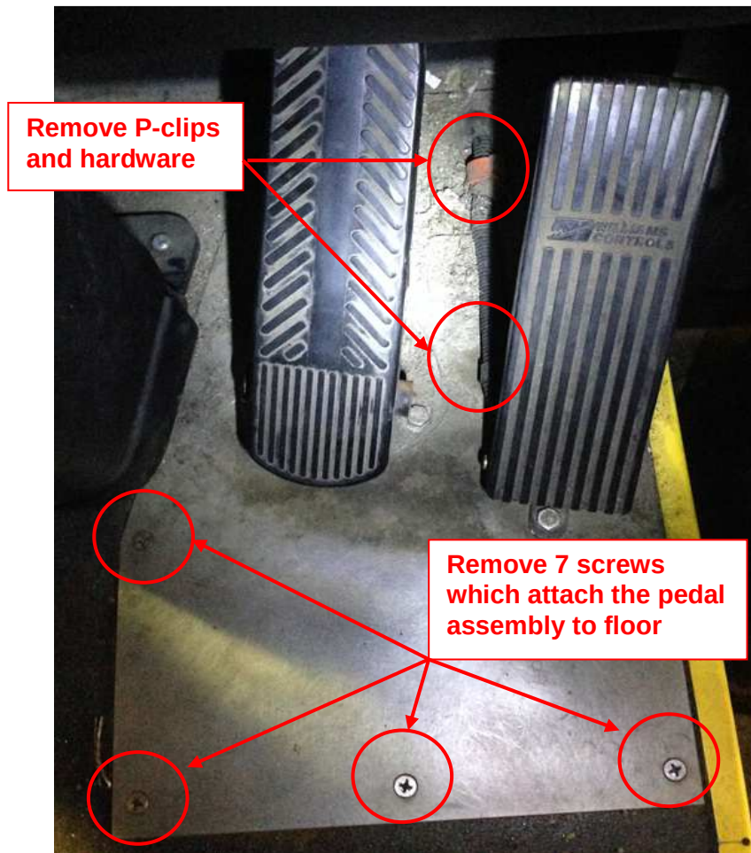
Figure 2: Brake/Accelerator Treadle Assembly
