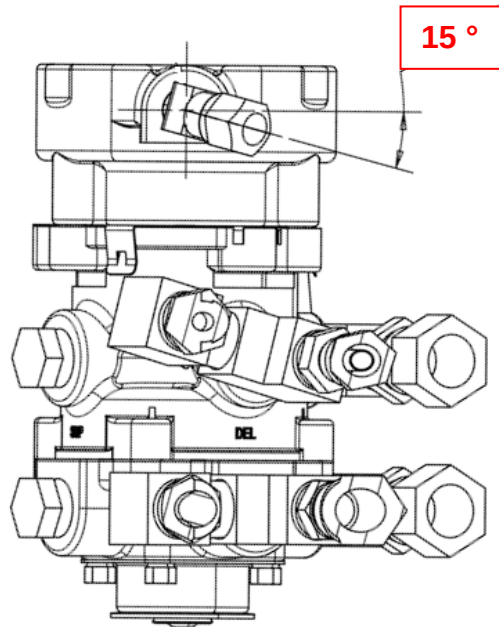
Figure 9: Align the 45 Degree Elbow
