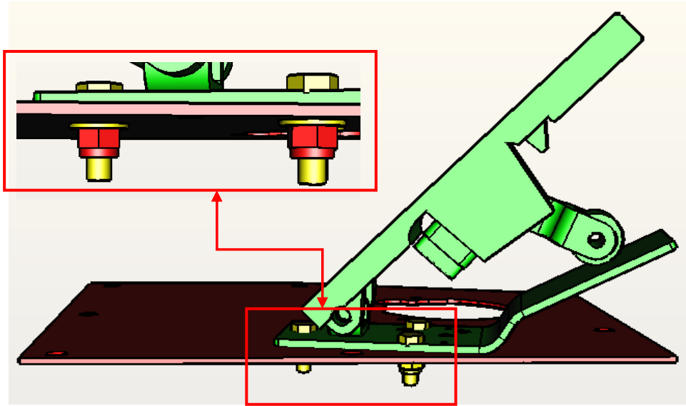
Figure 10(b): Install Accelerator Treadle
