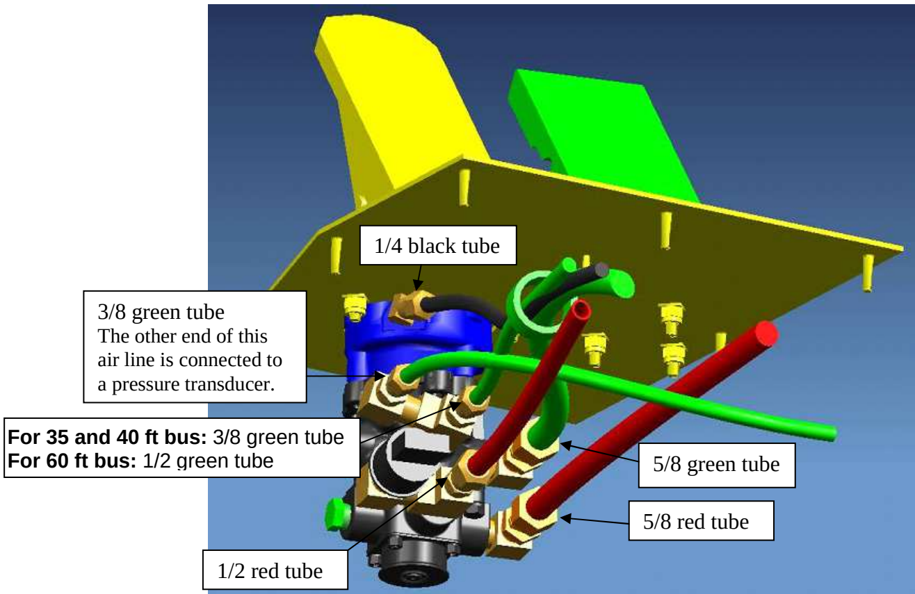
Figure 22: Airline Connections to the E6 and BVA Valves
