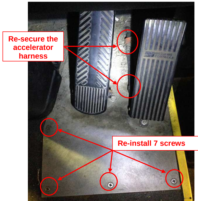
Figure 21: Brake/Accelerator Treadle Assembly
