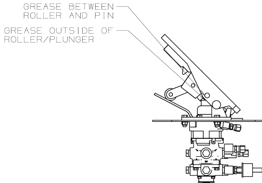
Figure 19: Apply Grease
