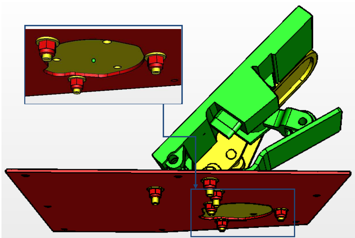
Figure 13: Pedal Mount
