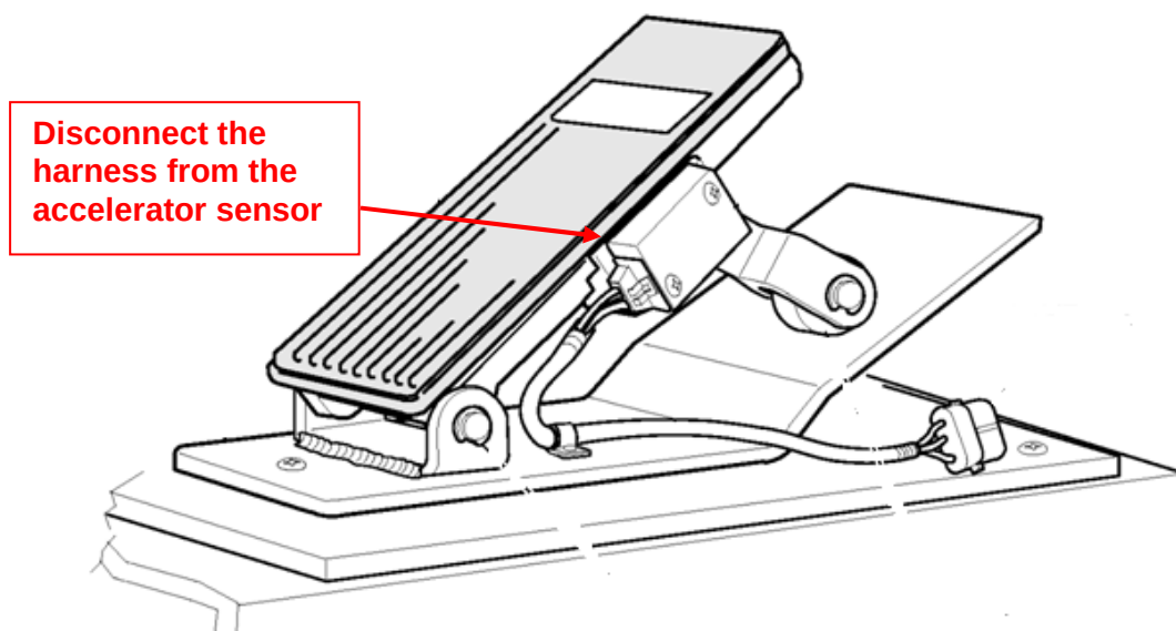
Figure 3: Brake/Accelerator Treadle Assembly
