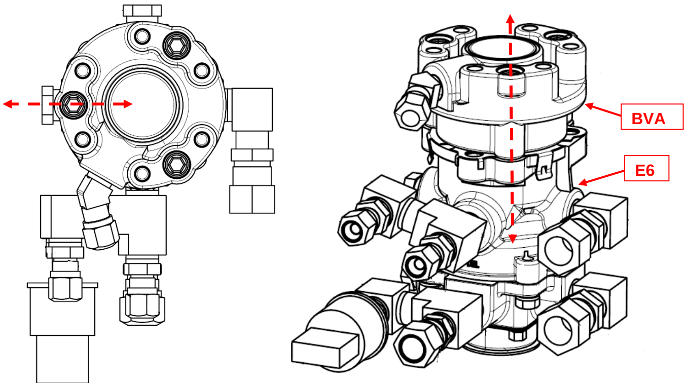
Figure 8: Replace BVA Valve
