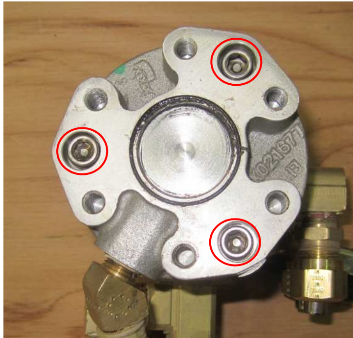
Figure 7: Remove BVA Valve
