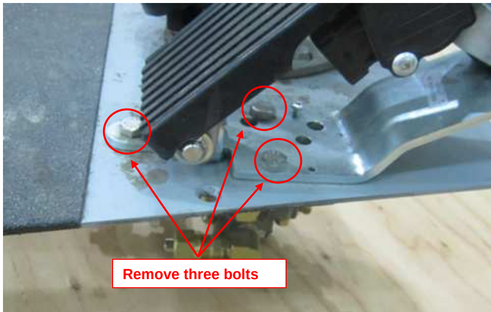
Figure 4: Remove Accelerator Treadle Assembly
