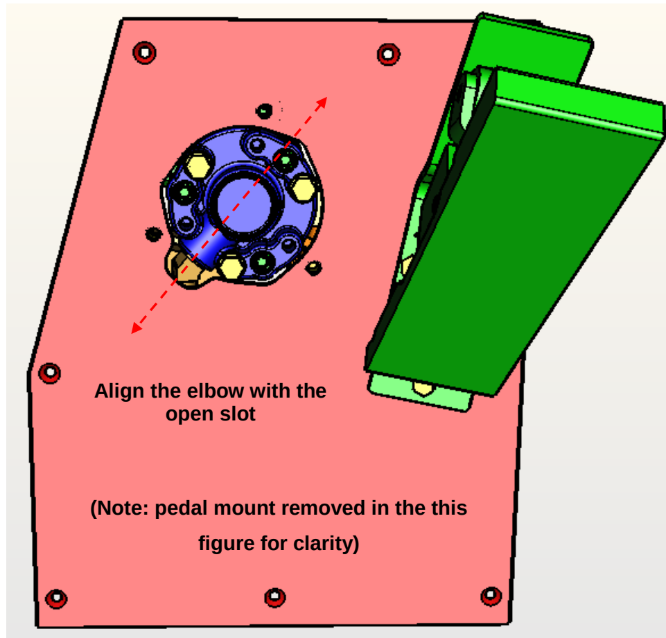
Figure 14: Align the BVA Valve with the New Plate
