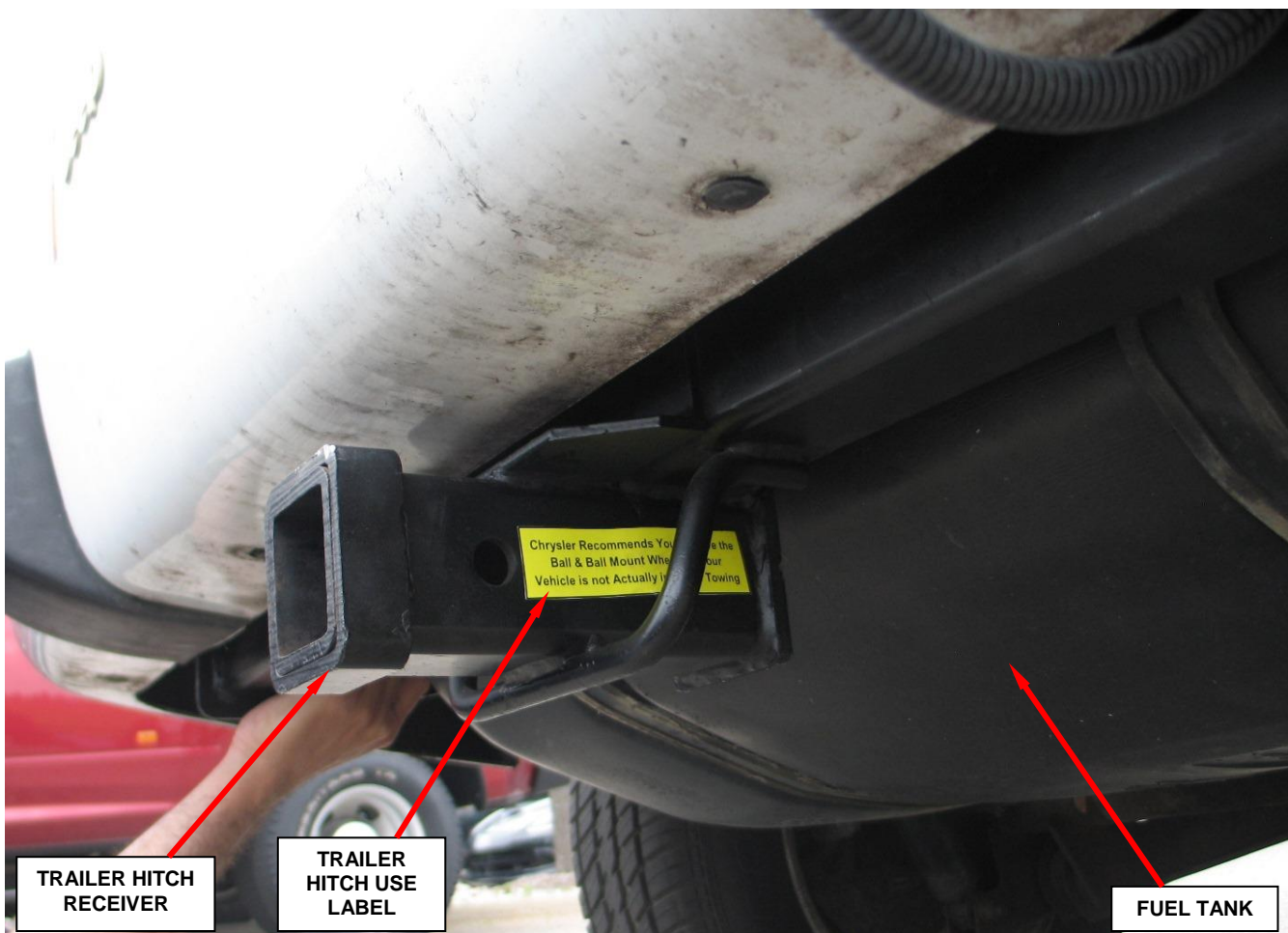
Figure 12 - Install Label on Right or Left Side of Trailer Hitch Receiver
